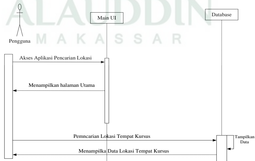
Gambar IV.7 Sequence Diagram Pembina
