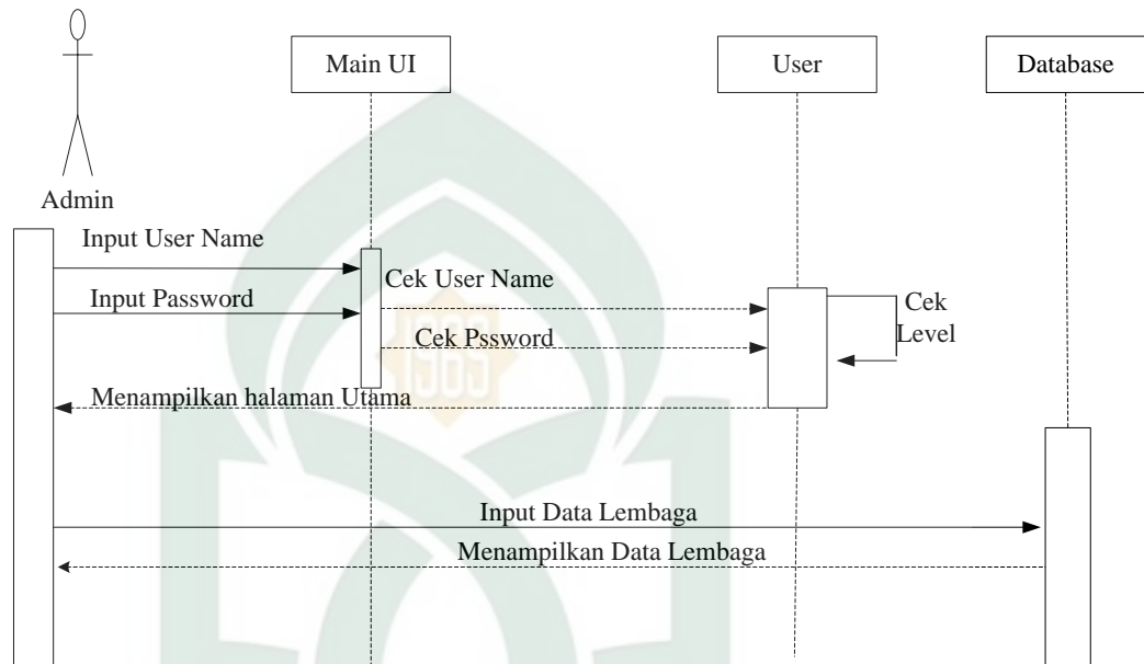
Gambar IV.6 Sequence Diagram Admin
