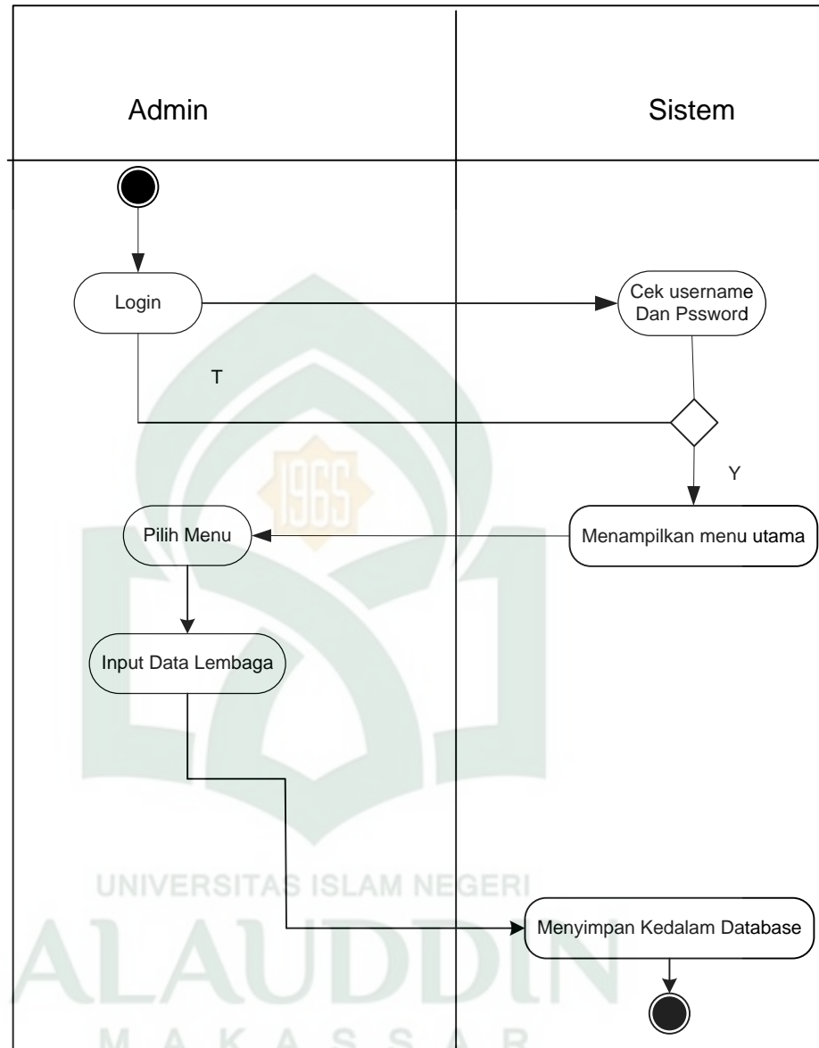
Gambar IV.4 Activity diagram
