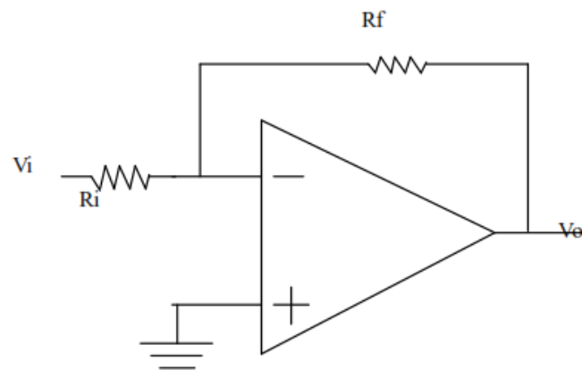
Gambar II.3 Penguat Inverting
