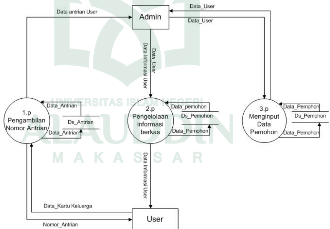
Gambar IV.5. Data Flow Diagram Level 1
