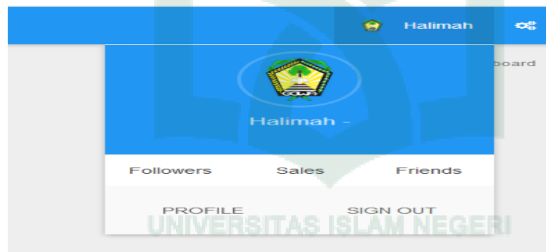
Gambar V.13 Logout
