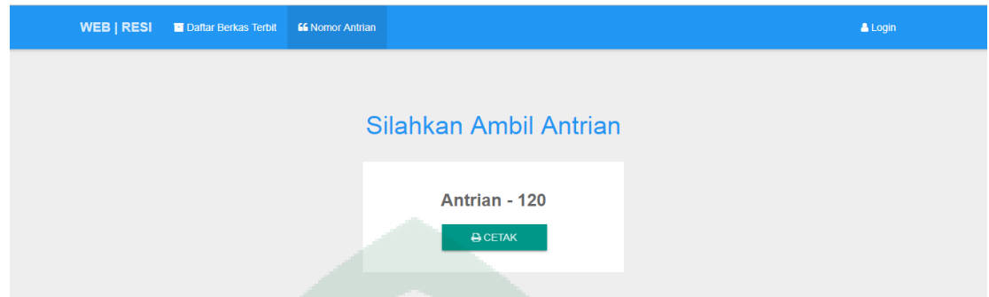
Gambar V.12 Nomor Antrian
