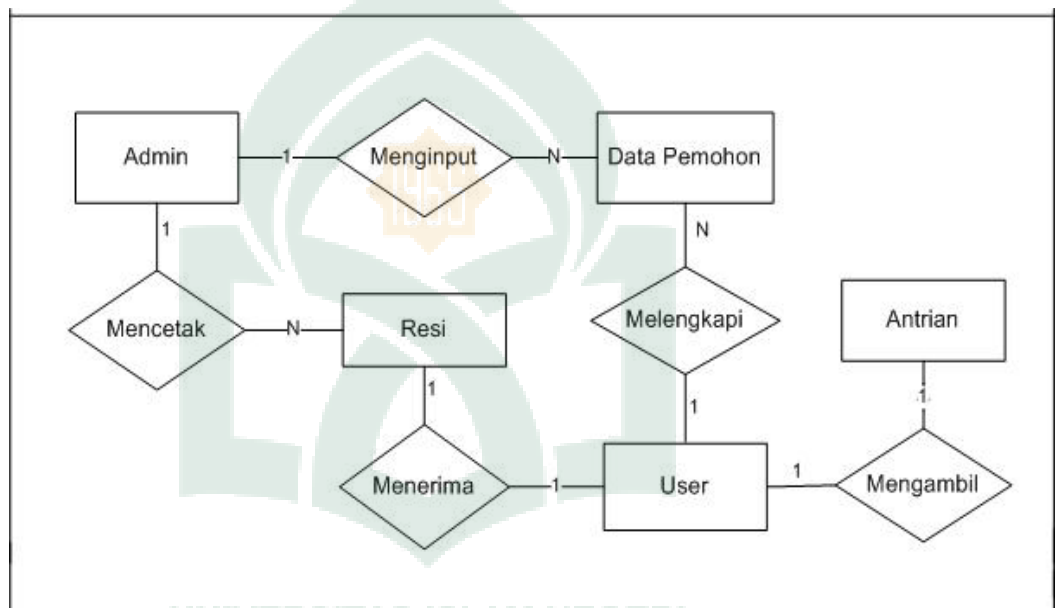
Gambar IV.7. Entity Relationship Diagram
