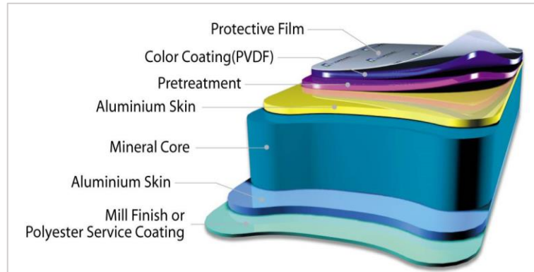
Gambar III.36. Bagian-Bagian Aluminium Composit Panel (ACP) Sumber: Alustaraluminium, 2019
