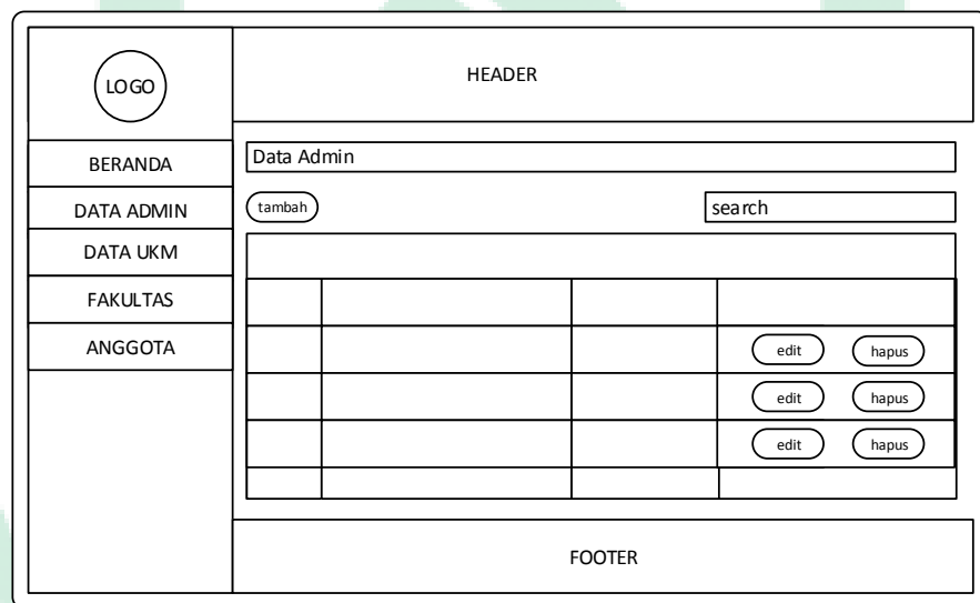
Gambar IV.24. Interface Data Admin
