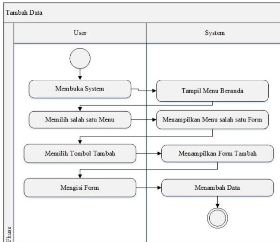
Gambar IV.14. Activity Diagram Tambah Data
