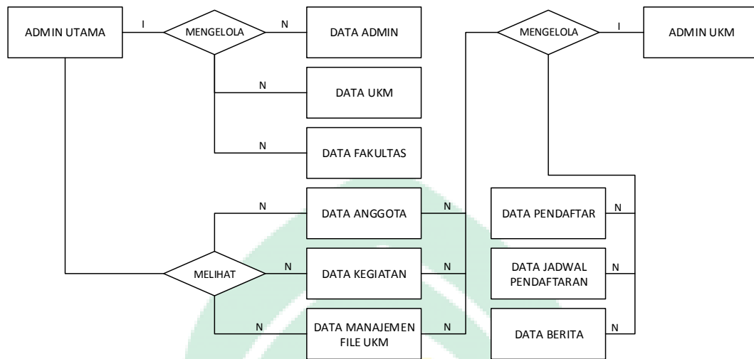
Gambar IV.21. Entity Relationship Diagram (ERD) Admin
