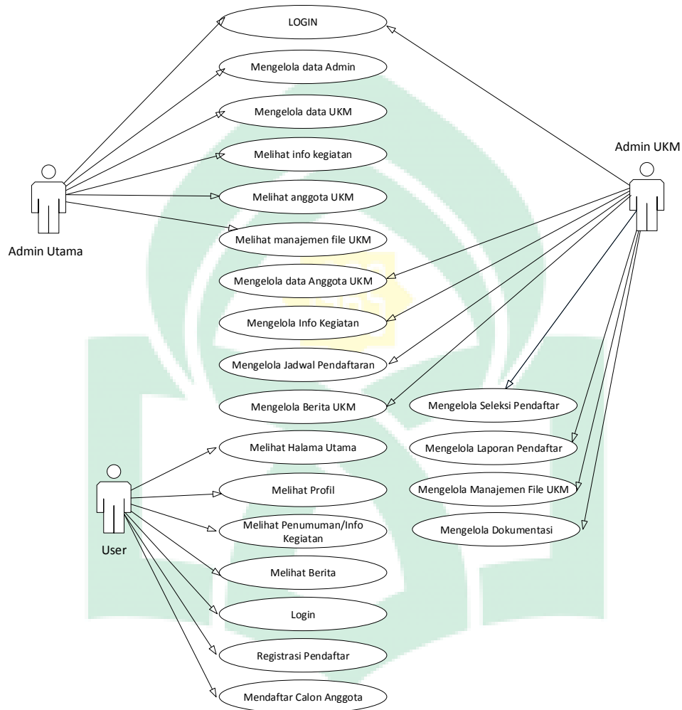
Gambar IV.3. Use Case Diagram
