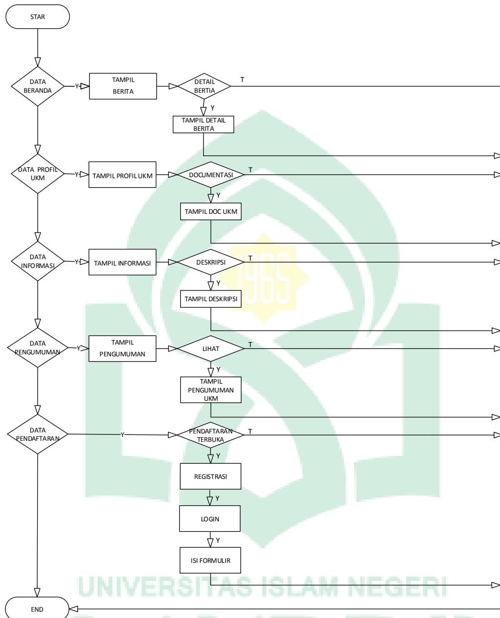
Gambar IV.20. Flowchart User
