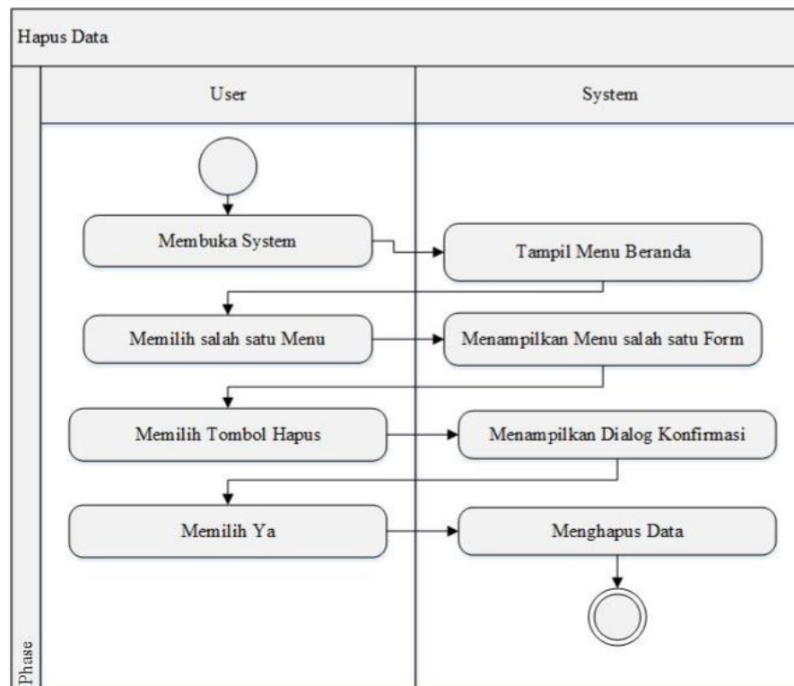
Gambar IV.16. Activity Diagram Hapus Data
