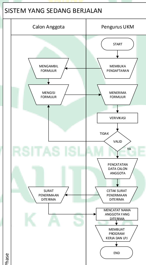
Gambar IV.1. Flowmap Diagram
