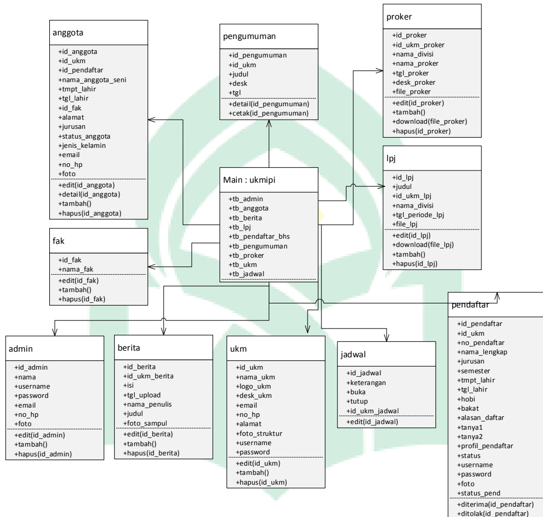
Gambar IV.4. Class Diagram
