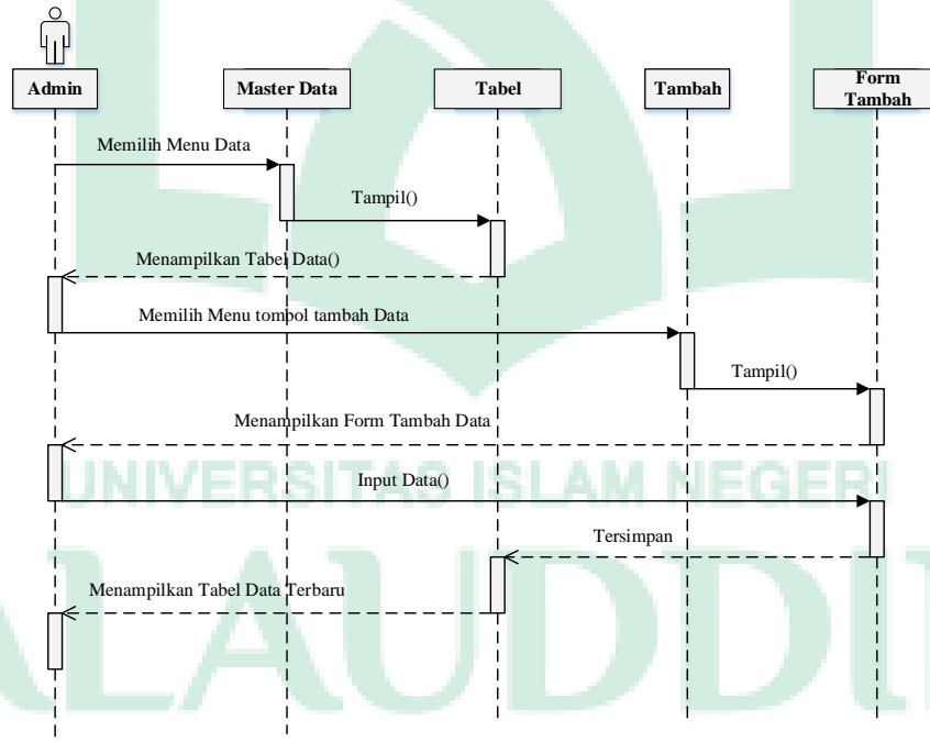
Gambar IV.8. Sequence Diagram Tambah Data
