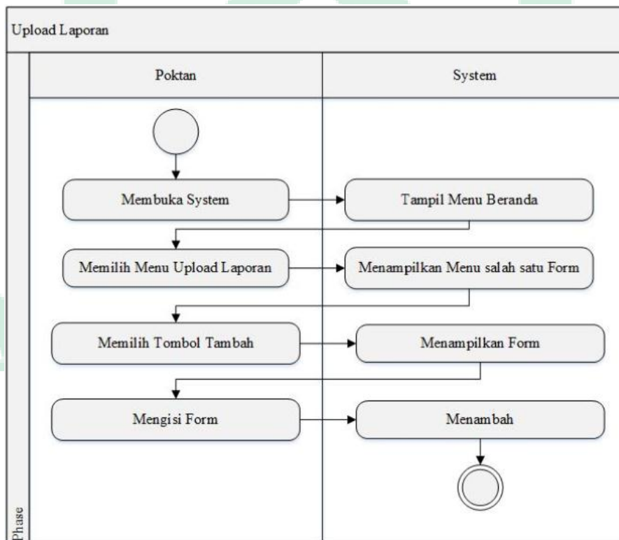
Gambar IV.17. Activity Diagram Upload Data
