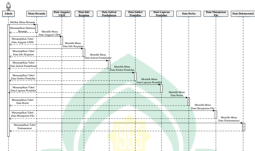
Gambar IV.7. Sequence Diagram Admin UKM
