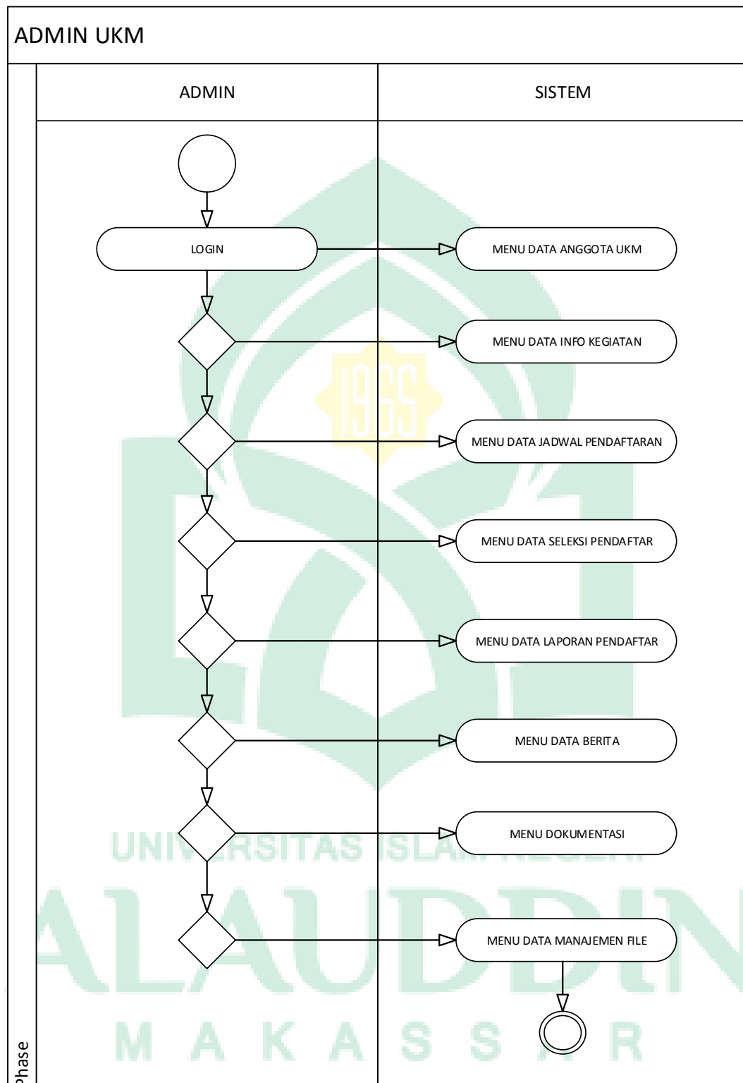
Gambar IV.13. Activity Diagram Admin UKM
