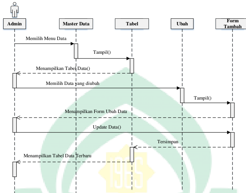
Gambar IV.9. Sequence Diagram Edit Data
