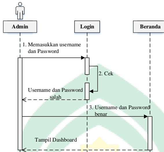
Gambar IV.5. Sequence Diagram Login Admin
