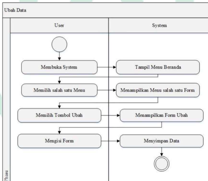
Gambar IV.15. Activity Diagram Ubah Data
