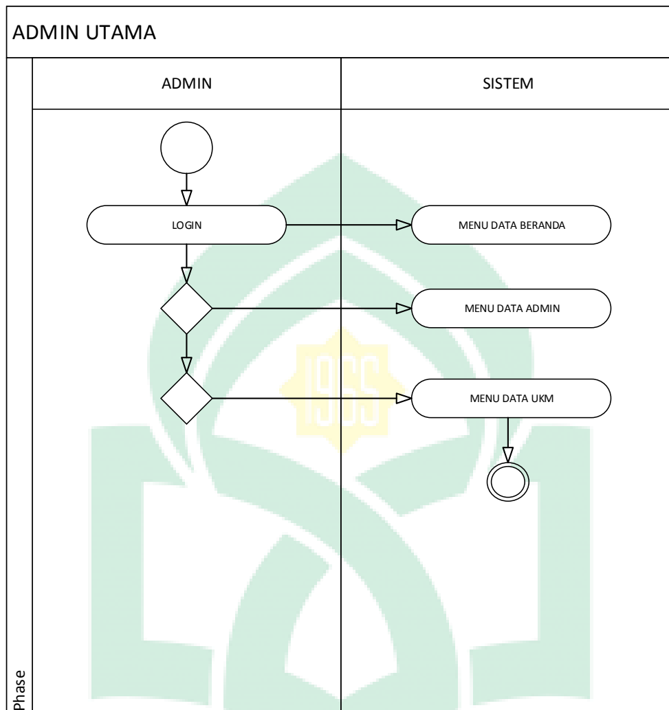
Gambar IV.12. Activity Diagram Admin Utama
