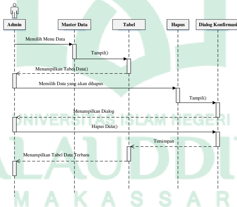
Gambar IV.10. Sequence Diagram Hapus Data
