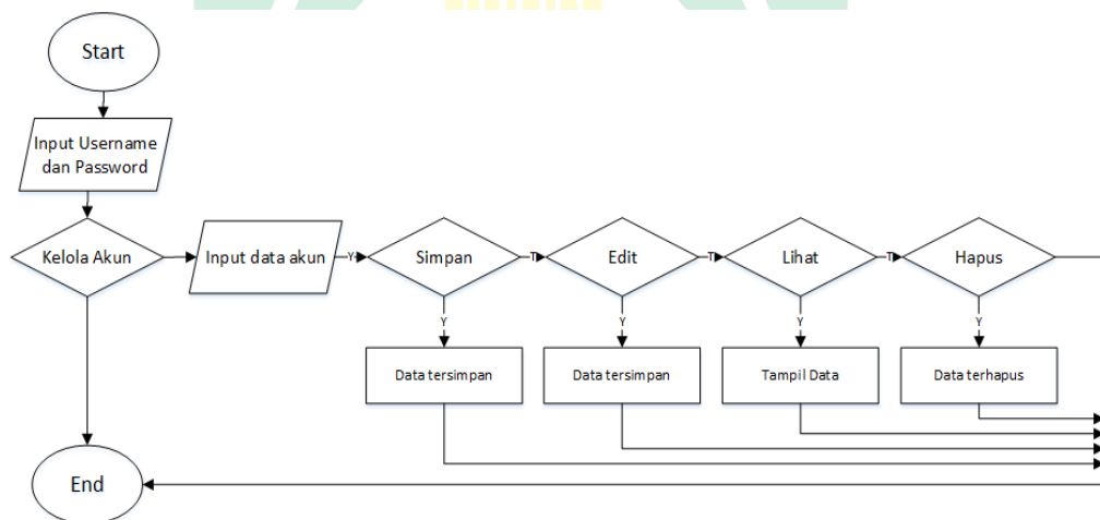
Gambar IV.3 Flowchart Admin
