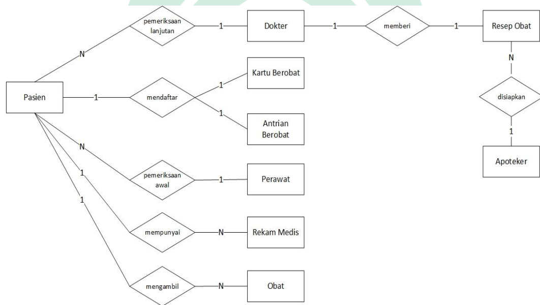
Gambar IV.13 Entity Relationship Diagram
