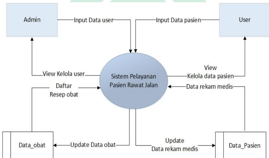
Gambar IV.9 Diagram level 0
