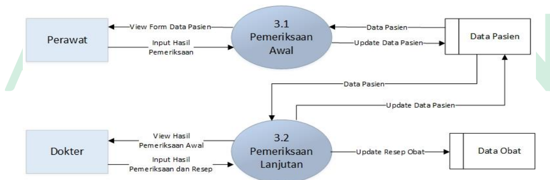
Gambar IV.12 Diagram level 2.2
