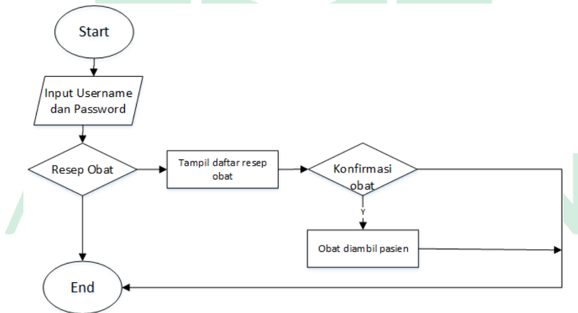
Gambar IV.7 Flowchart Apoteker
