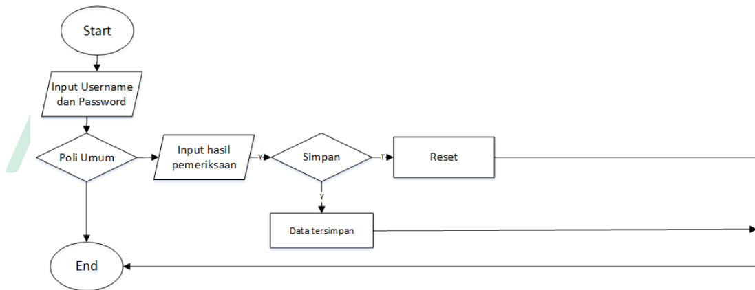
Gambar IV.5 Flowchart Perawat
