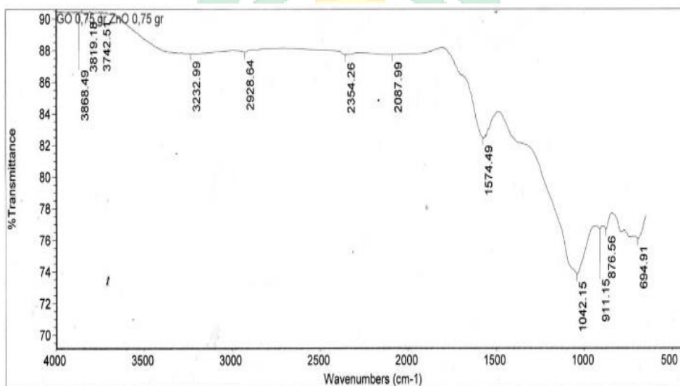
Gambar 4.6 Grafik FTIR rGO-ZnO
