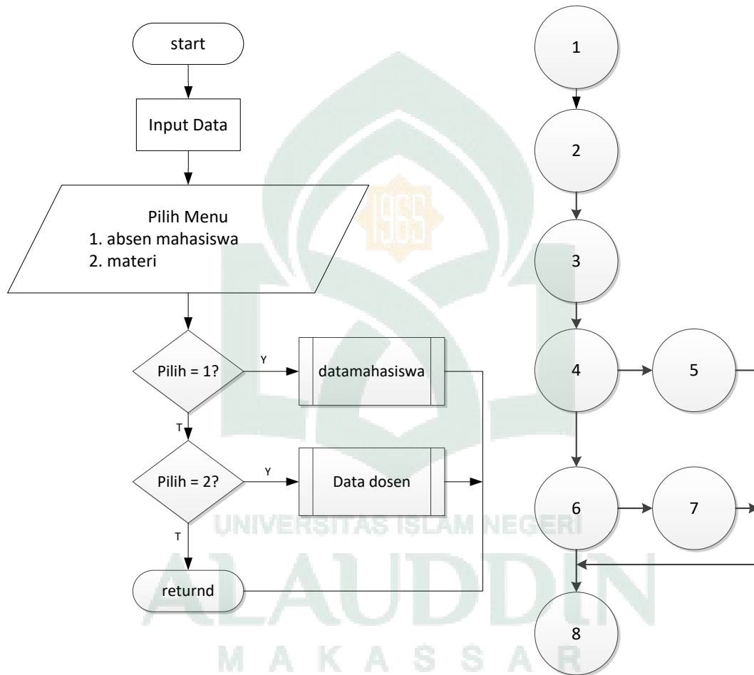
Gambar V. 10. Flowchart dan Flowgraph Halaman Dosen Input Data
