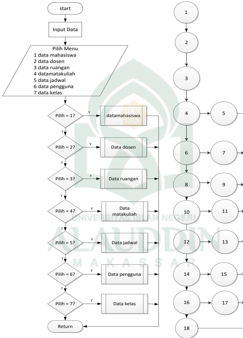
Gambar V. 7. Flowchart dan Flowgraph Input Data Admin
