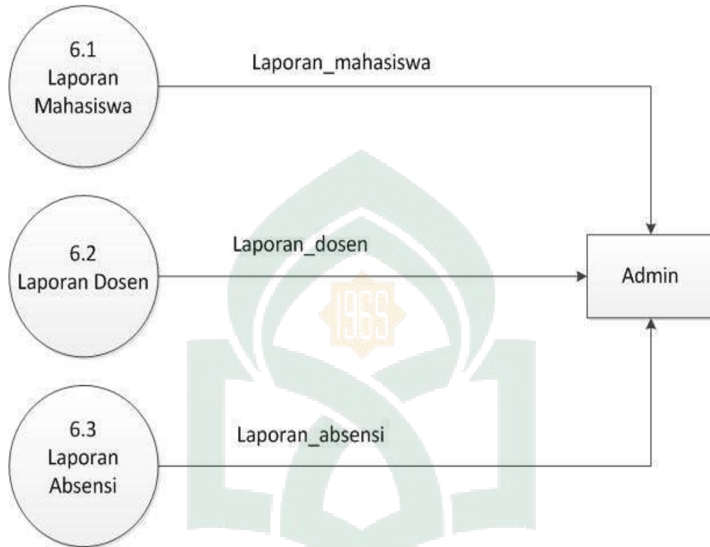
Gambar IV. 6. Diagram Level 2 Proses 6
