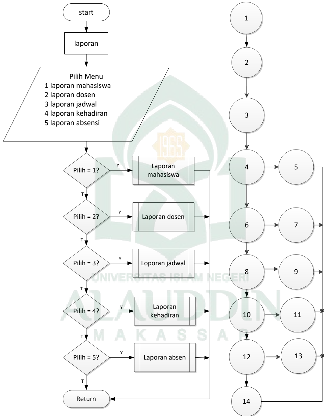
Gambar V. 8. Flowchart dan Flowgraph Laporan Admin
