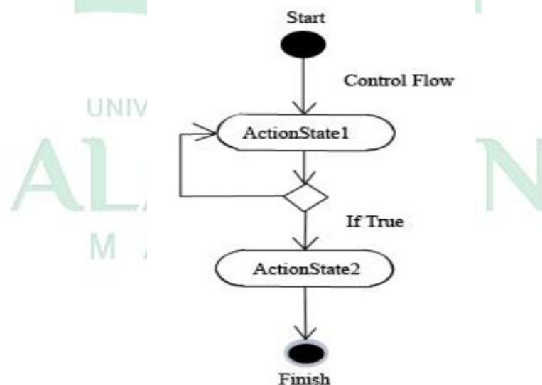
Gambar II.4 Model Activity Diagram (Darwiyanti,2003)
