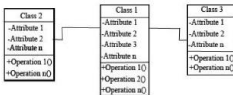
Gambar II.5 Model class diagram (munawar, 2005)
