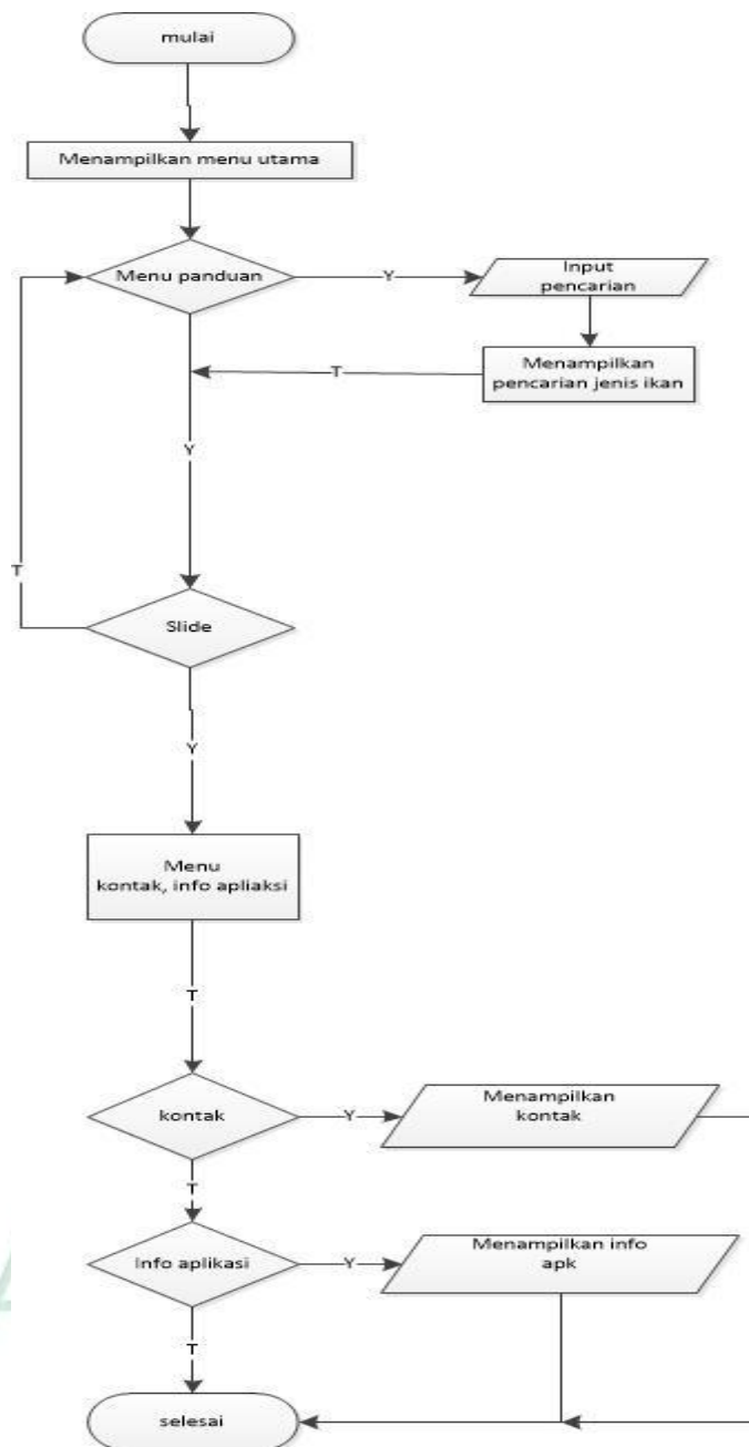
Gambar IV.12 Flowchart (Alur Program) User
