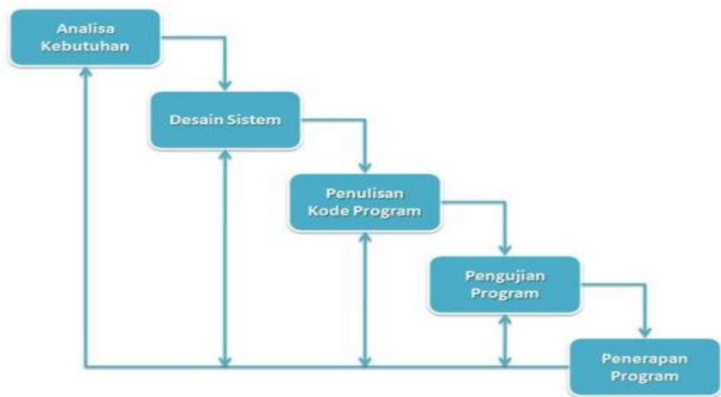
Gambar III.1: Model Waterfall
