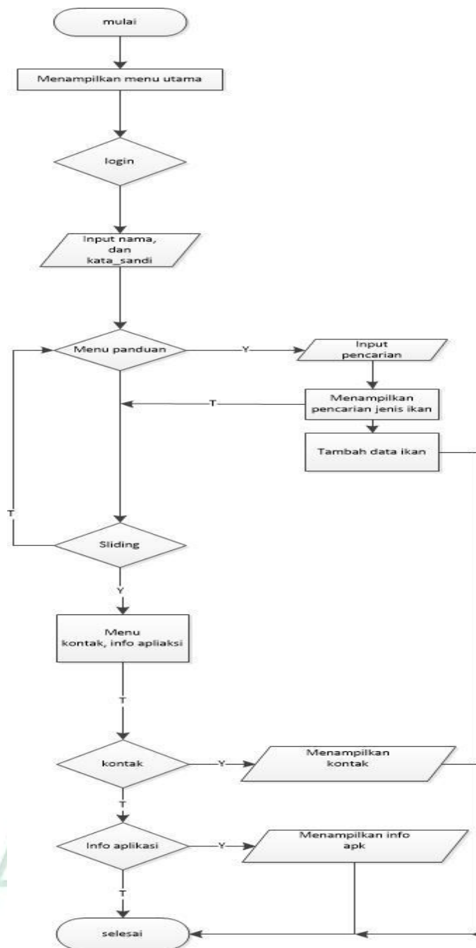
Gambar IV.13 Flowchart (Alur Program) Admin
