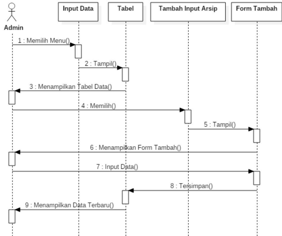
Gambar IV.9 Sequence diagram input arsip
