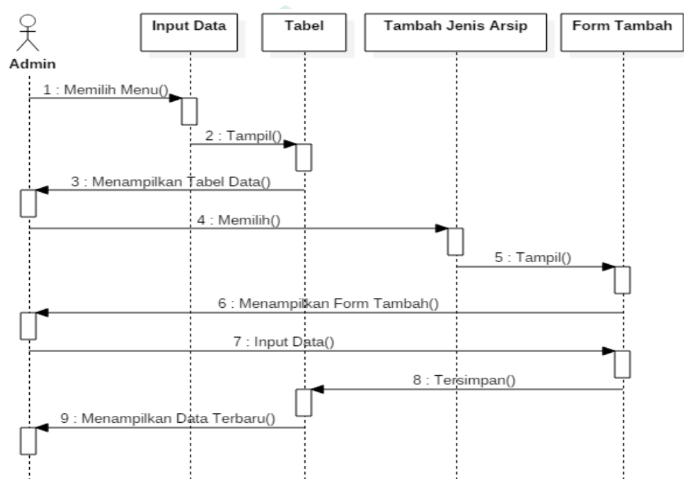
Gambar IV.7 Sequence diagram input data jenis arsip
