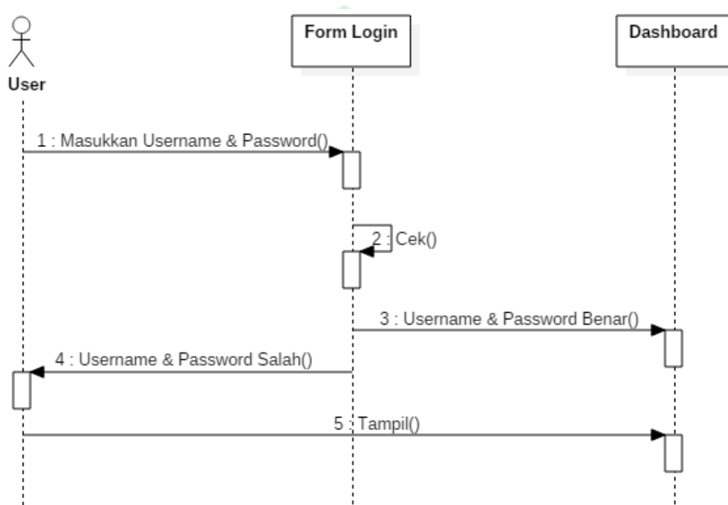
Gambar IV.4 Sequence Diagram login
