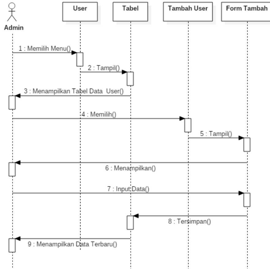
Gambar IV.10 Sequence diagram mengelola user
