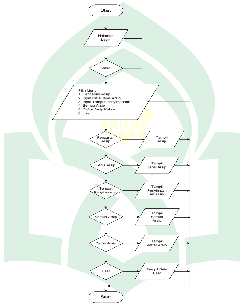
Gambar 1V.14 Flowchart
