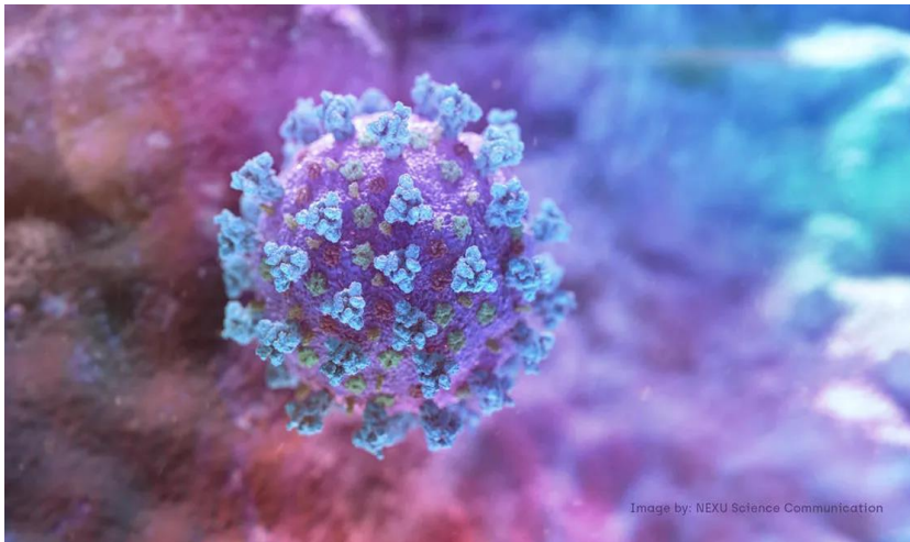
Gambar 8. Virus SAR-COV-2 78
