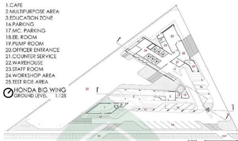
Gambar II.30. Site plan Honda Big Wing Bangkok (Sumber: https://www.archdaily.com/146543/honda-big-wing-vaslab-architecture , diakses pada tanggal 17 September 2018)
