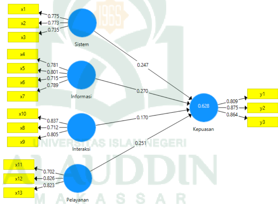
Gambar 4.3 Model Akhir Penelitian
