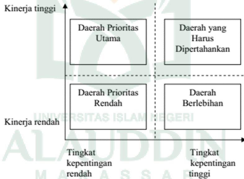
Gambar 2.1 Diagram Importance Performance Analysis
