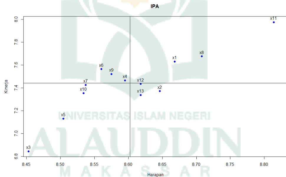
Gambar 4.2 Diagram Importance Performance Analysis
