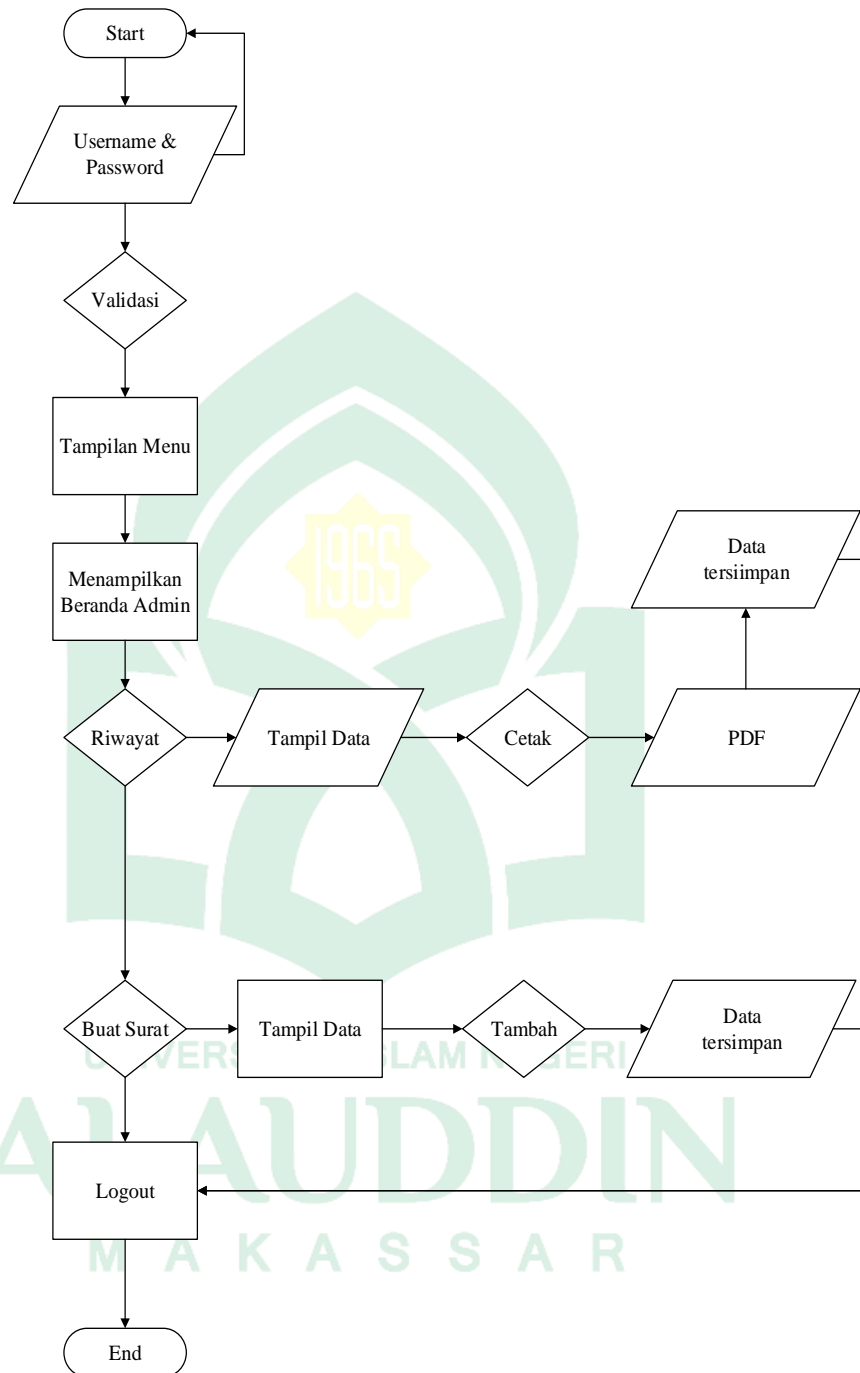
Gambar IV. 20 Flowchart staf
