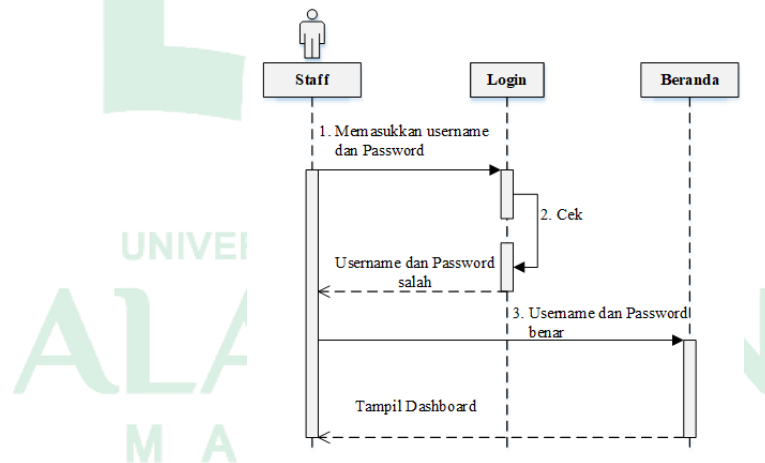
Gambar IV. 7 Sequence Diagram Login Staf
