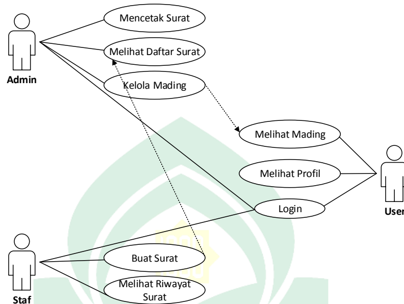
Gambar IV.4 Use Case Diagram
