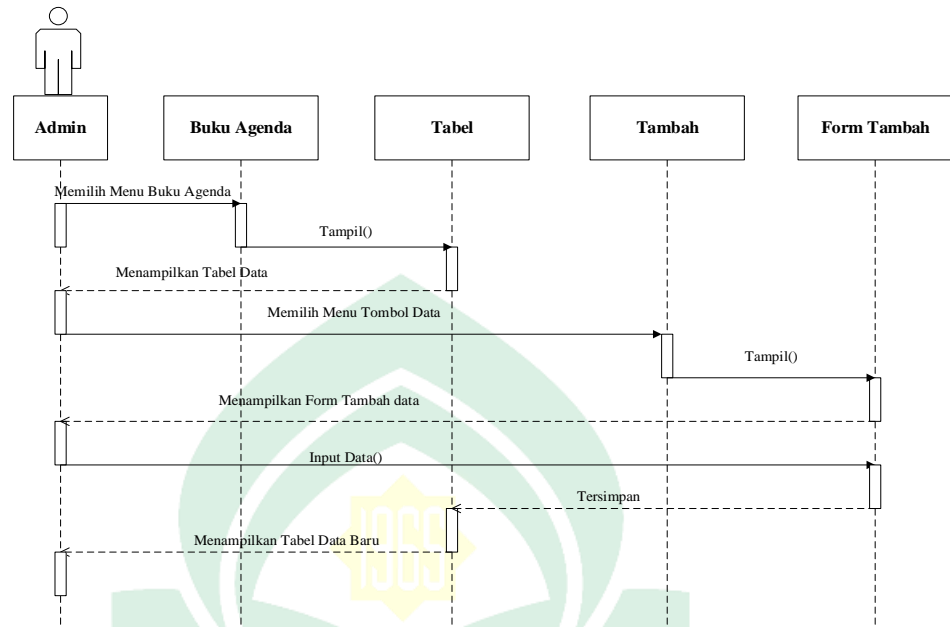
Gambar IV. 8 Sequence Diagram Tambah Data
