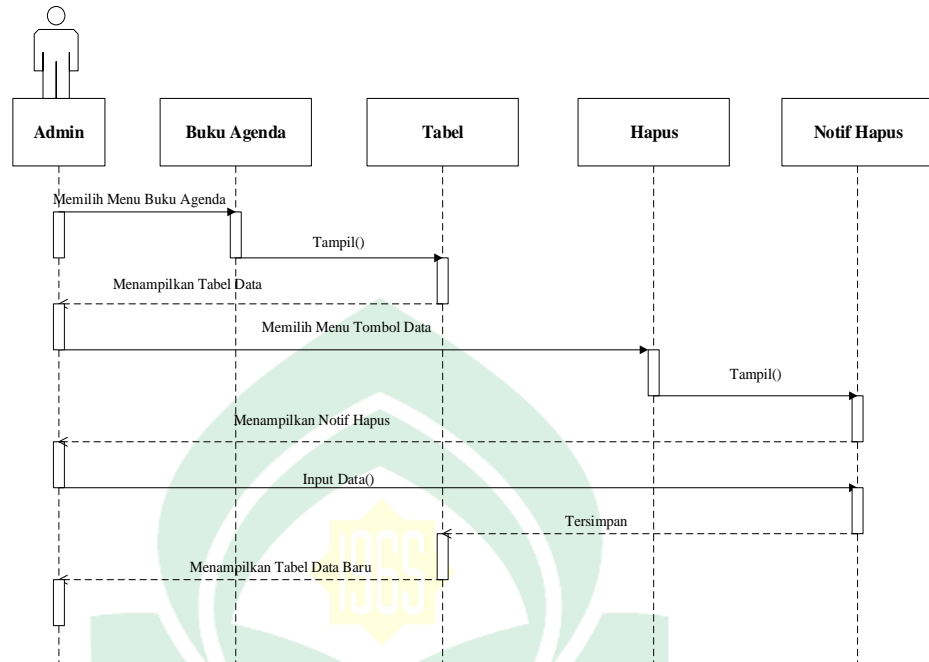
Gambar IV. 10 Sequence Diagram Hapus Data
