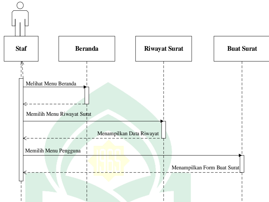
Gambar IV. 12 Sequence Diagram Menu Staf
