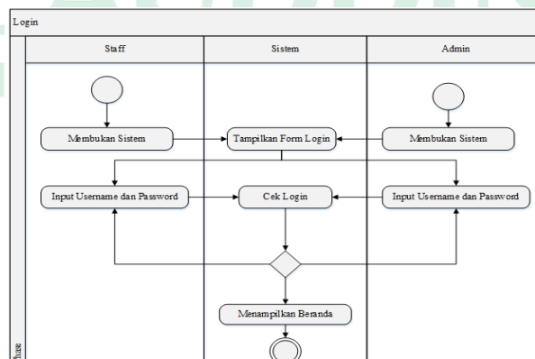
Gambar IV. 13 Activity Diagram Login
