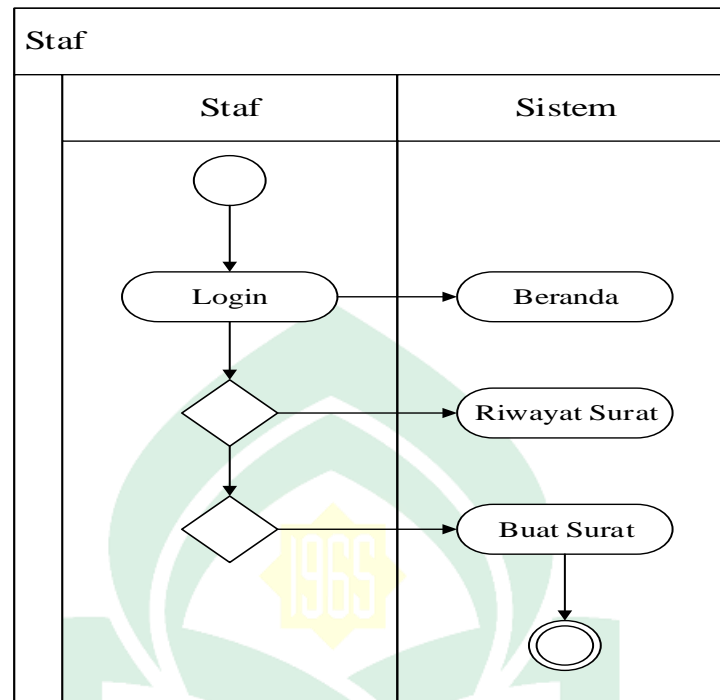
Gambar IV.18 Activity Diagram Menu Staf
