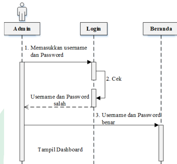
Gambar IV. 6 Sequence Diagram login Admin
