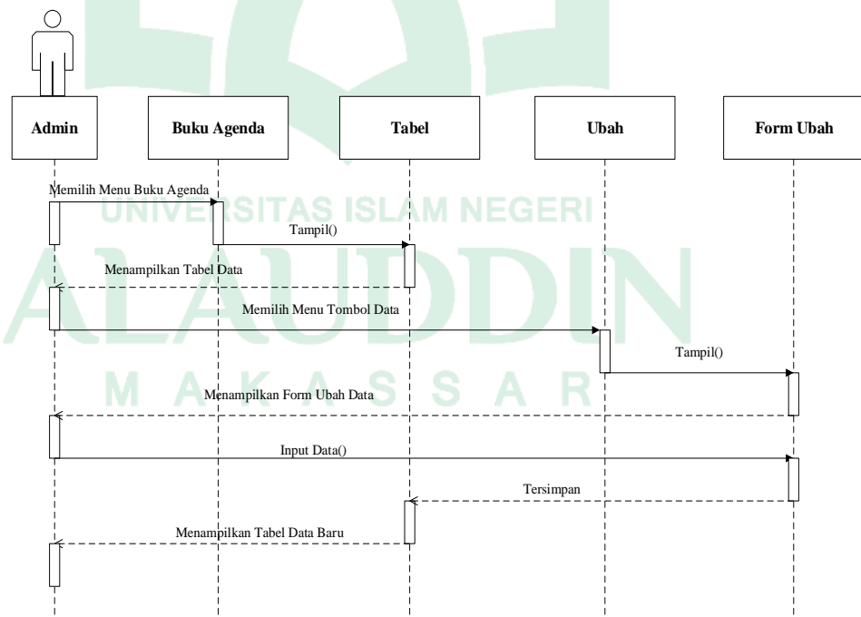
Gambar IV. 9 Sequence Diagram Update Data
