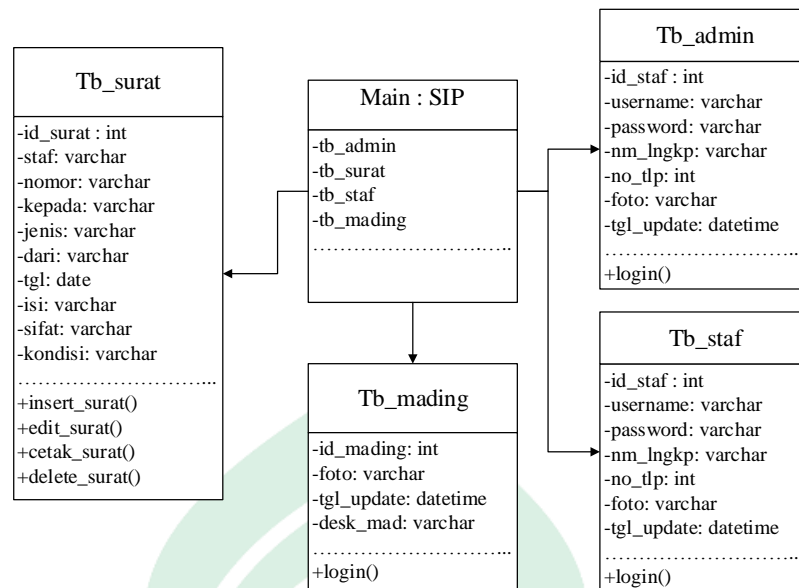
Gambar IV.5 Class Diagram
