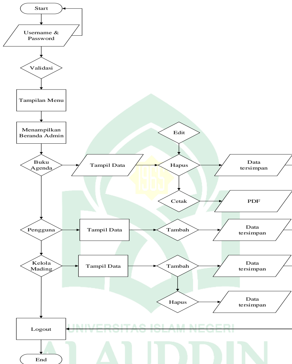
Gambar IV.19 Flowchart Admin
