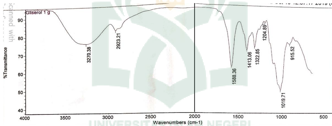
Gambar 4.7 Spektrum FTIR edible film penambahan gliserol 15%
