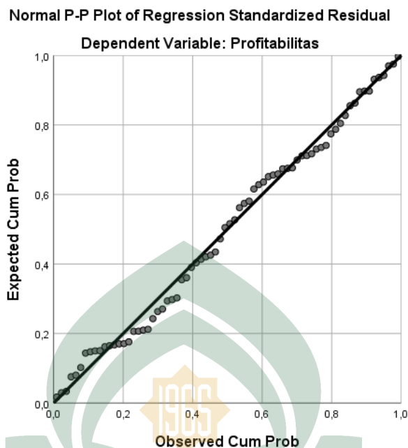
Gambar 4.2 Hasil Uji Normalitas – Normal Probability Plot
