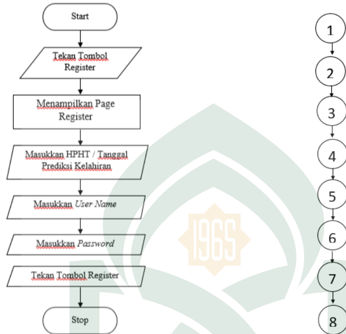
Gambar V.9 Flowchart dan Flowgraph Menu Register
