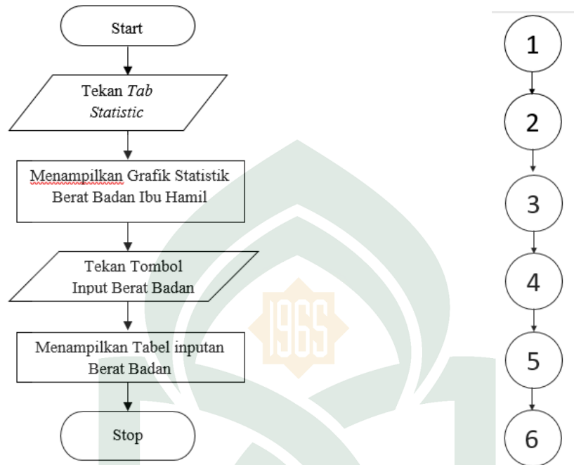
Gambar V.11 Flowchart dan Flowgraph Menu Statistic
