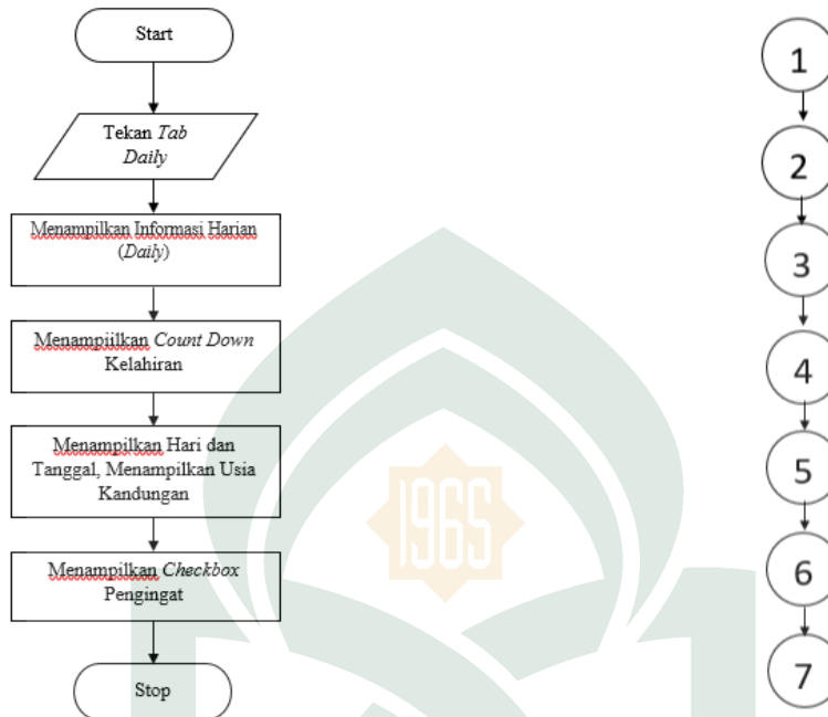
Gambar V.10 Flowchart dan Flowgraph Menu Daily
