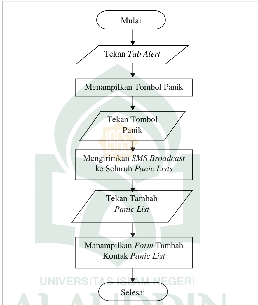
Gambar IV.10 Flowchart Tab Alert
