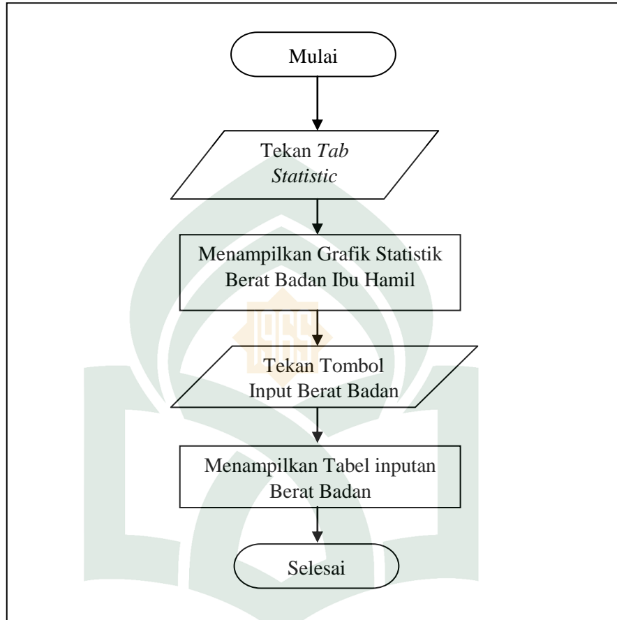
Gambar IV.9 Flowchart Tab Statistic
