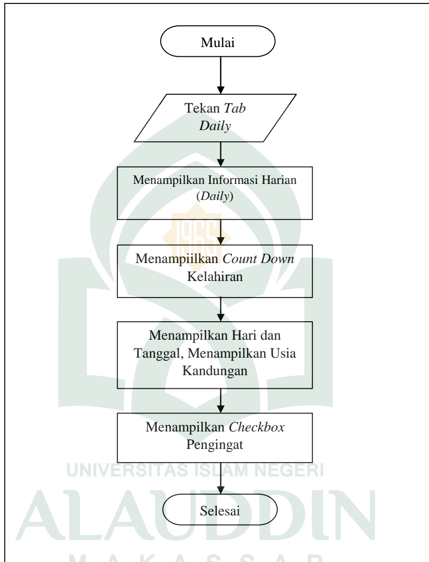
Gambar IV.8 Flowchart Tab Daily
