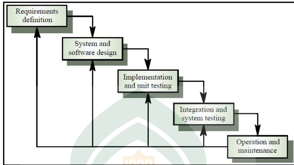
Gambar III.1 Metode Waterfall
