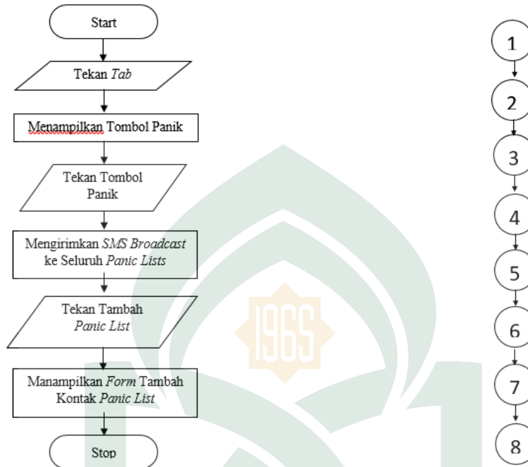
Gambar V.12 Flowchart dan Flowgraph Menu Panic Button
