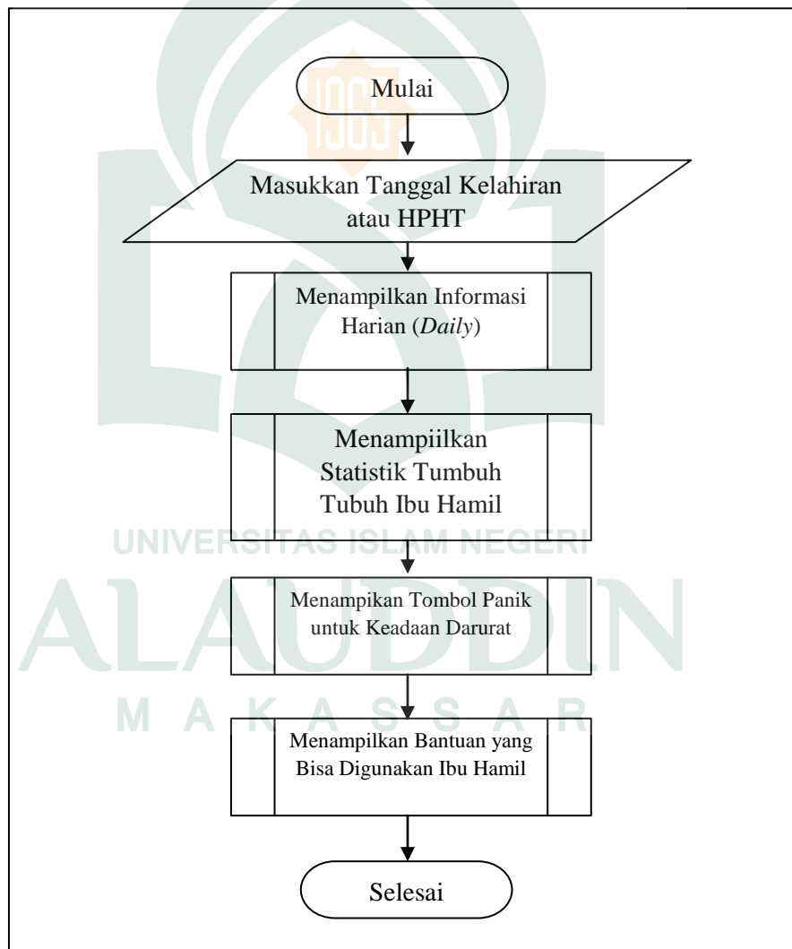
Gambar IV.7 Flowchart Sistem
