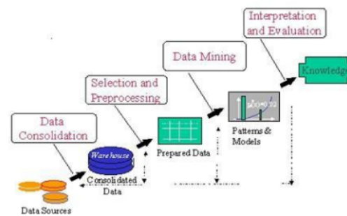
Figure 1: KDD process
