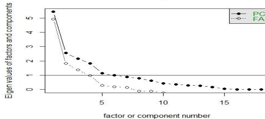
Scree plot
