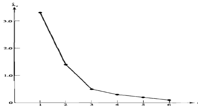
Gambar 2.1 Scree Plot
