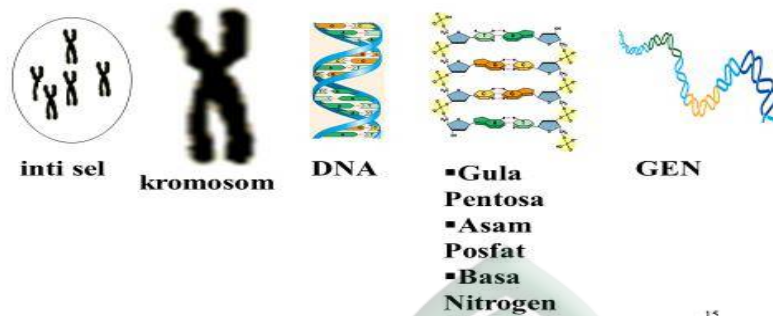
Figure 1. Cell-chromosomes-DNA-Nitrogenous Base-Gene
