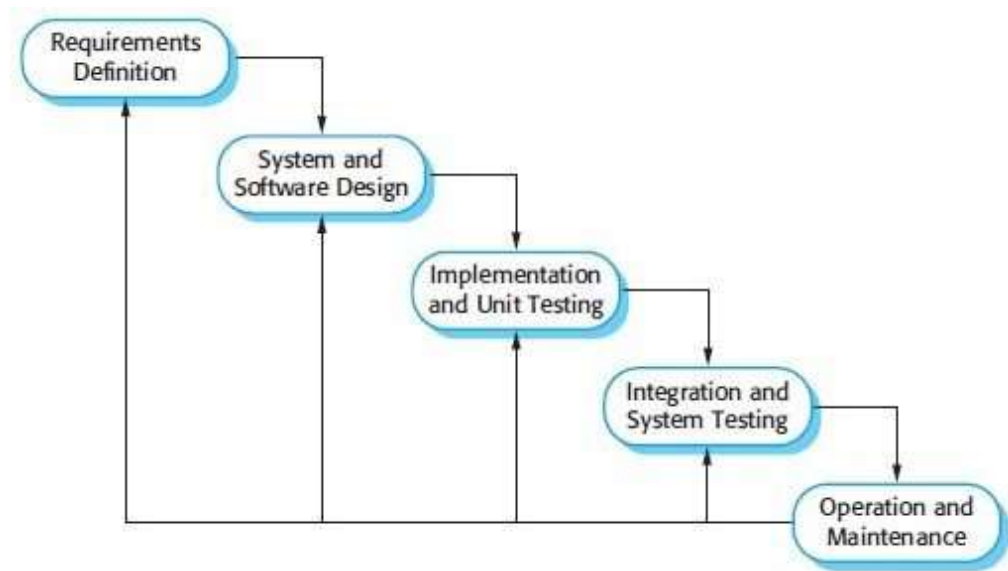
Gambar III. 1. Model Waterfall (Summerville 2011)
