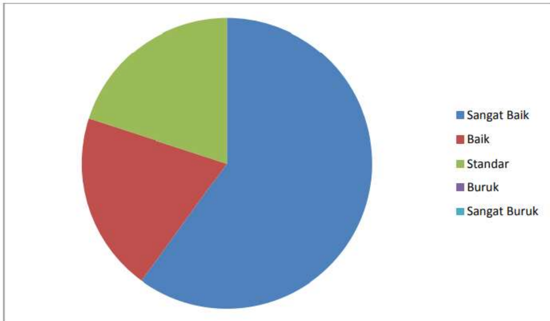
Gambar V.10 Diagram Kriteria 2
