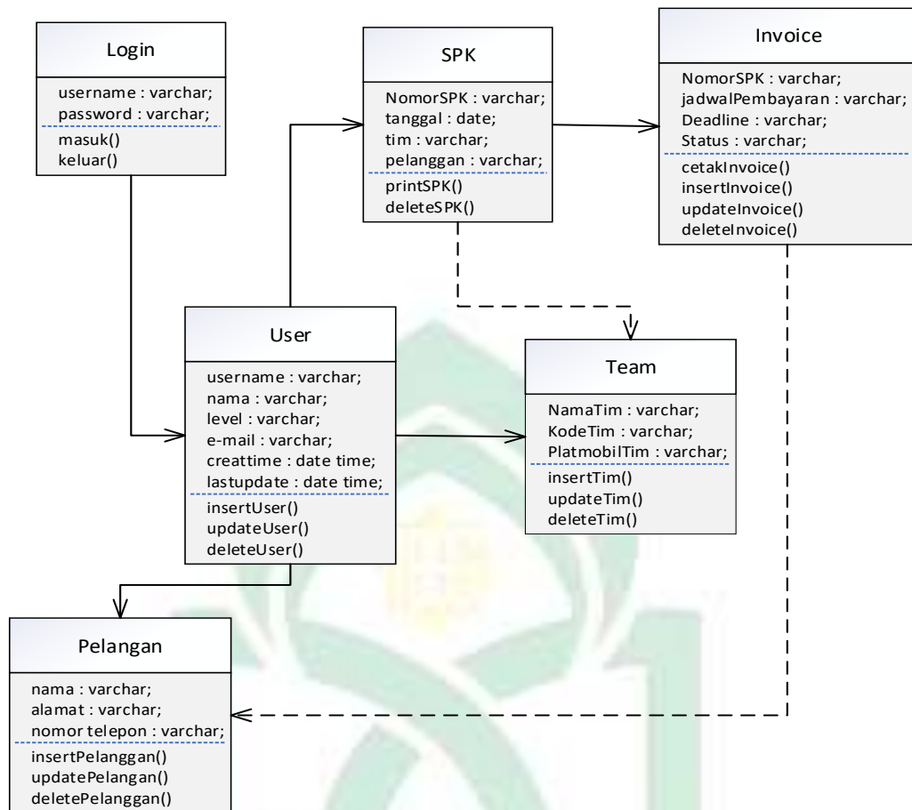
Gambar IV. 4 Class Diagram
