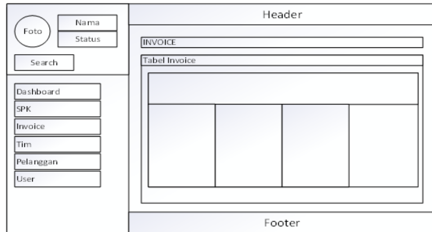
Gambar IV. 12 Antarmuka Invoice
