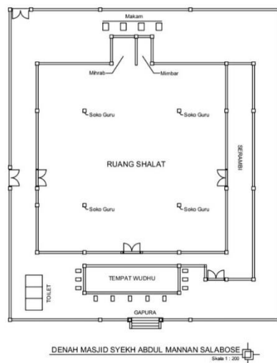
Gambar 18 Denah Masjid Tua Syekh Abdul Mannan
