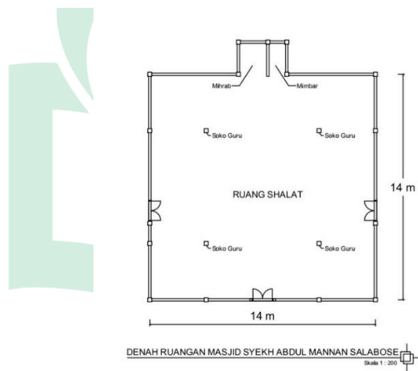
Gambar 19 Denah Ruang Peribadatan Masjid Tua Syekh Abdul Mannan
