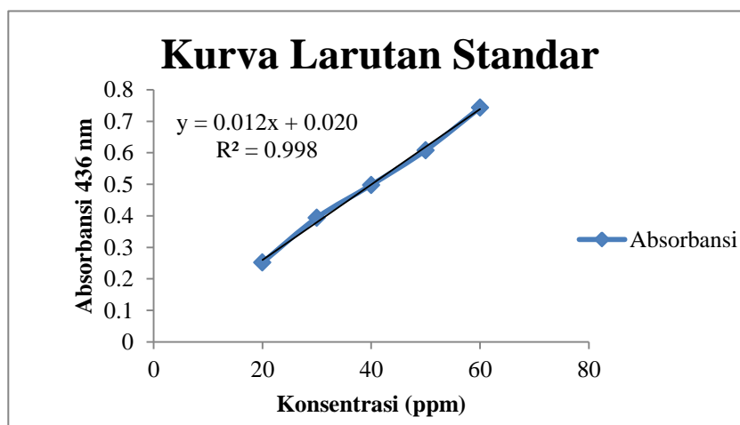
Gambar 3.7 Kurva Larutan Standar
