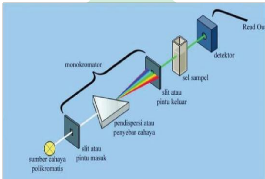
Gambar 2.6 Diagram alat spektrofotometer UV-Vis single-beam
