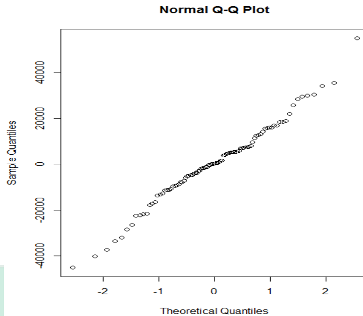
Gambar 4.10 Grafik Distribusi Normal Residual
