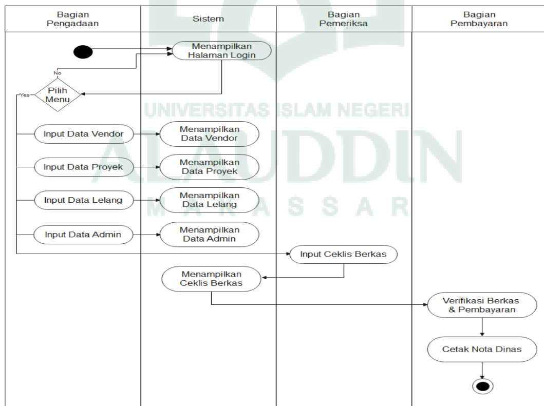
Gambar IV. 5 Activity Diagram Administrator
