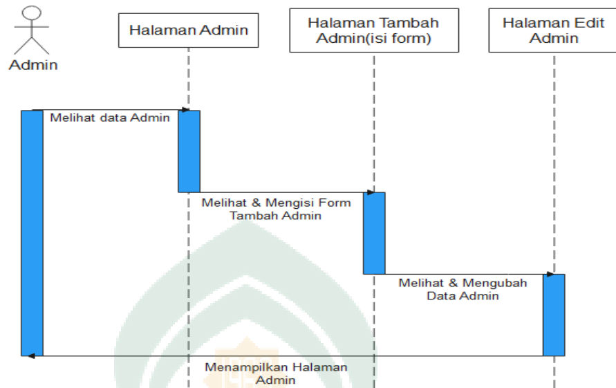
Gambar IV. 10 Sequence Diagram Admin
