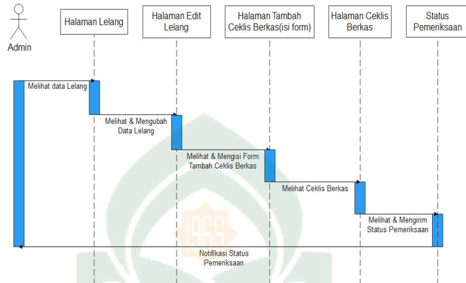
Gambar IV. 11 Sequence Diagram Lelang
