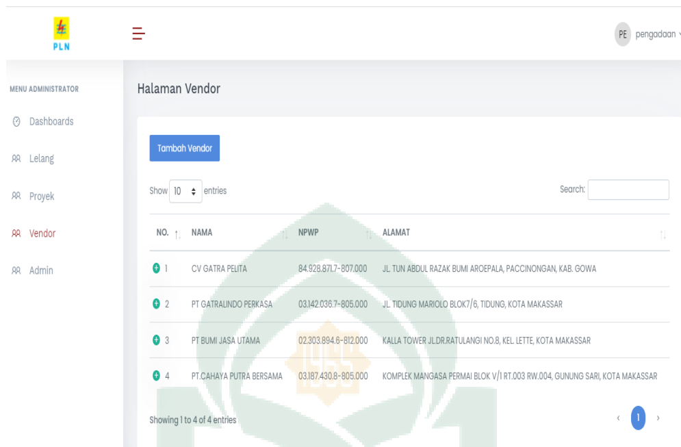
Gambar V. 2 Tampilan Halaman Vendor Pengadaan
