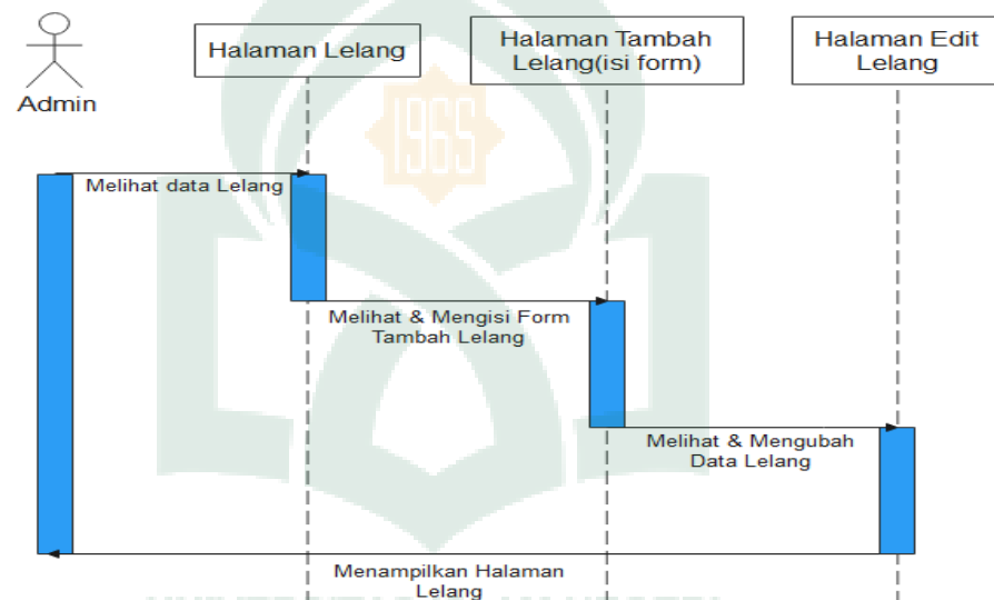
Gambar IV. 9 Sequence Diagram Lelang
