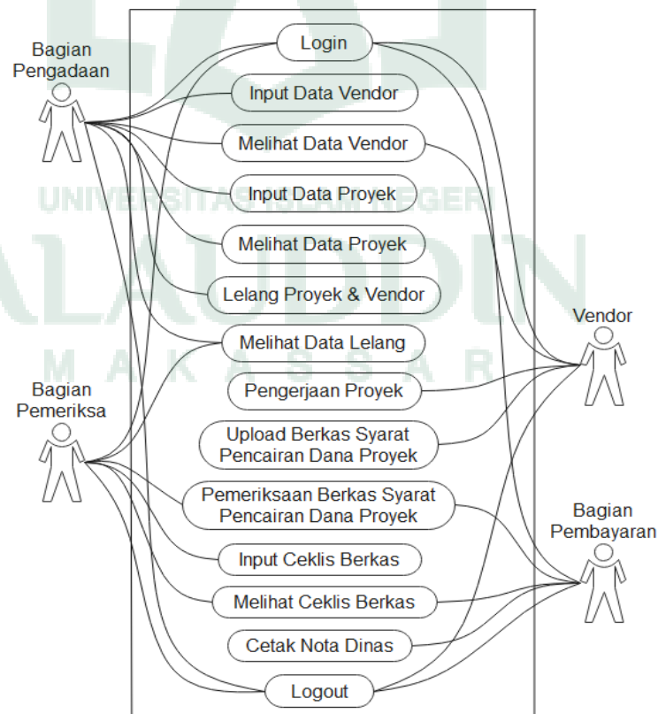
Gambar IV. 3 Use Case Diagram
