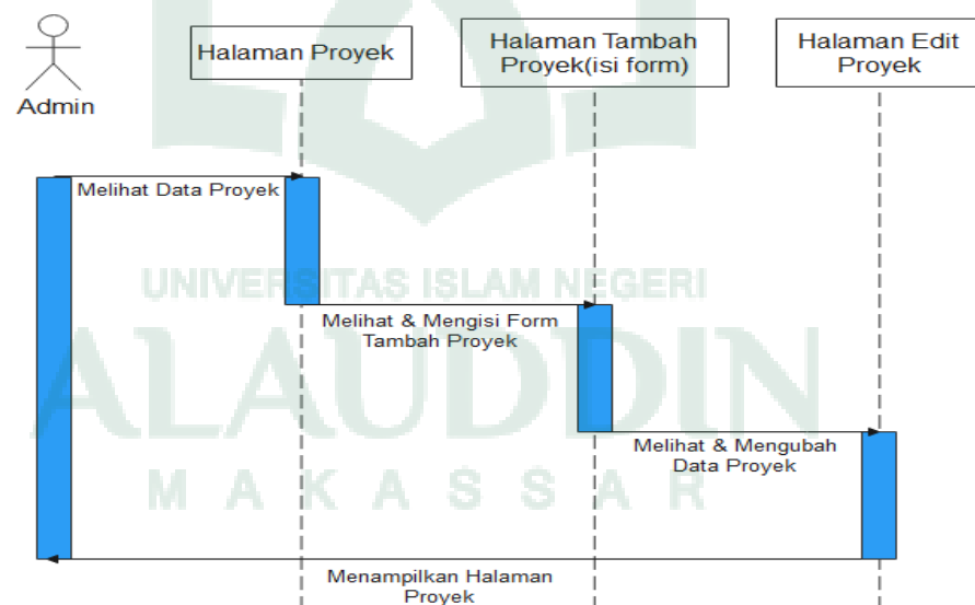
Gambar IV. 8 Sequence Diagram Proyek
