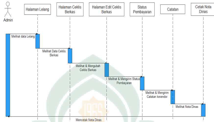
Gambar IV. 12 Sequence Diagram Lelang
