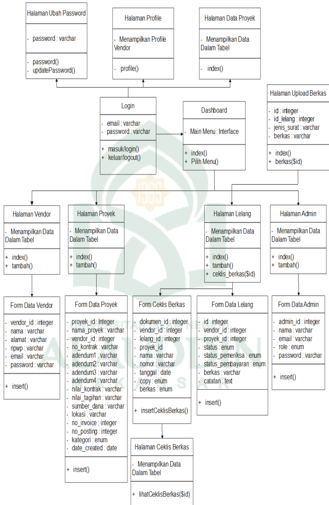
Gambar IV. 4 Class Diagram
