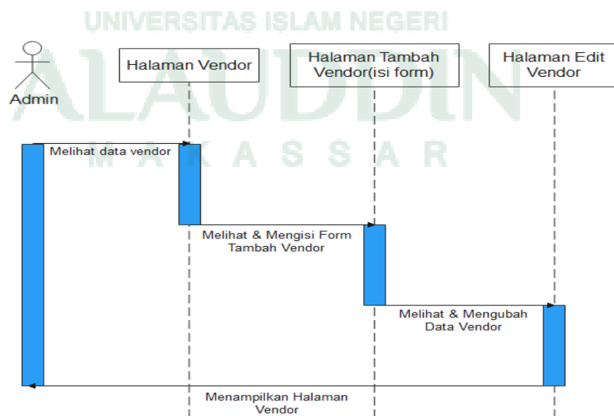
Gambar IV. 7 Sequence Diagram Vendor
