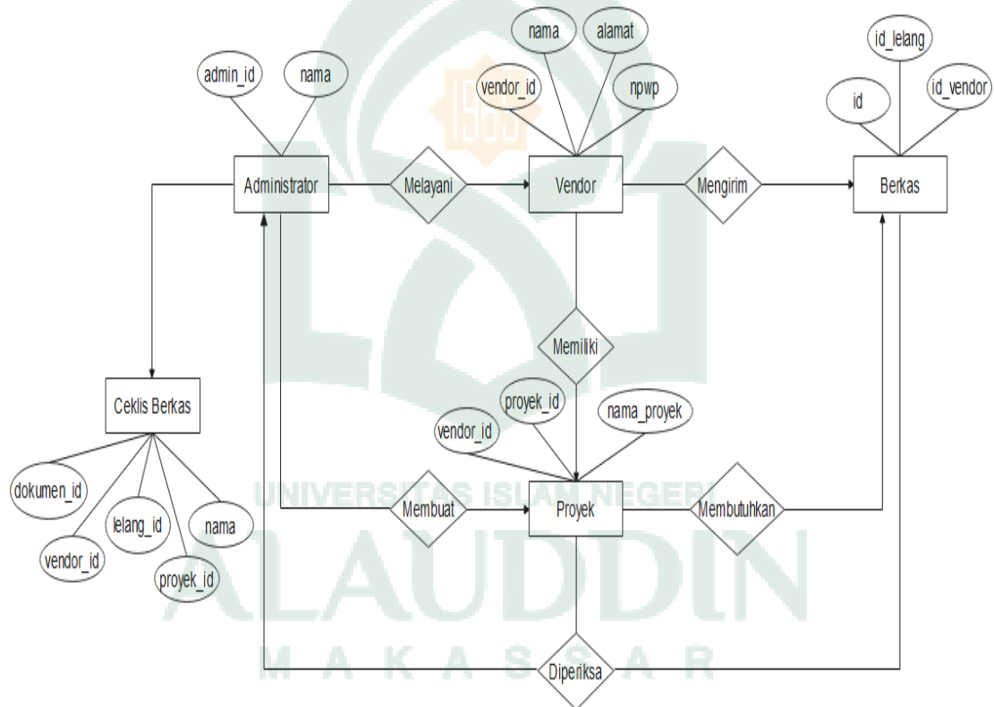
Gambar IV. 15 Diagram ERD
