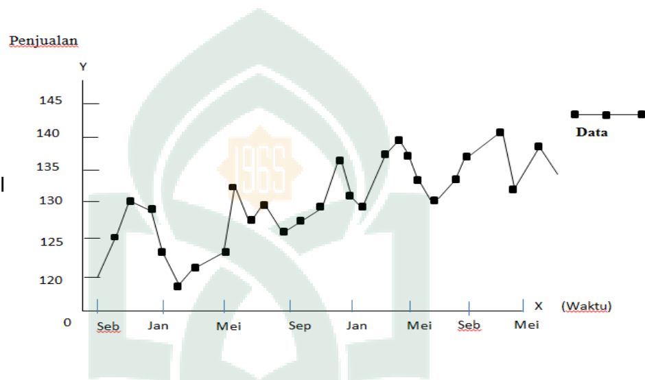
Gambar. 2.6. Double Moving Average kuartalan
