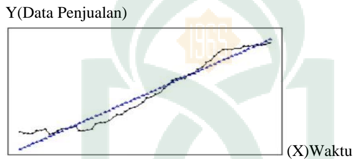
Gambar. 2.7. Double Exponential Smoothing Pola Trend
