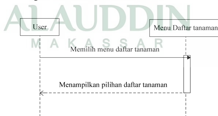
Gambar IV.7. Sequence Diagram Menu Daftar Tanaman
