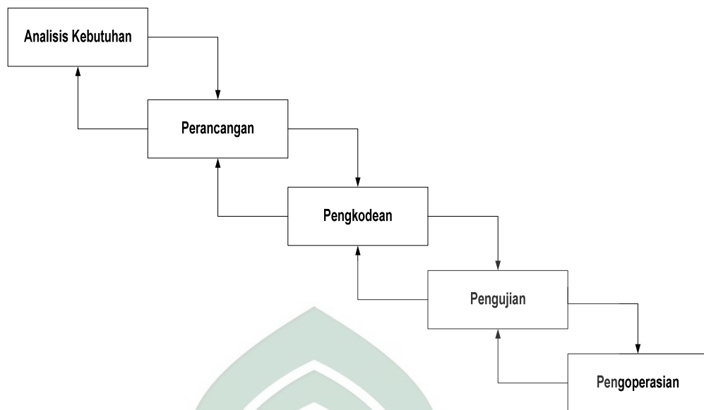
Gambar III.1. Model Waterfall
