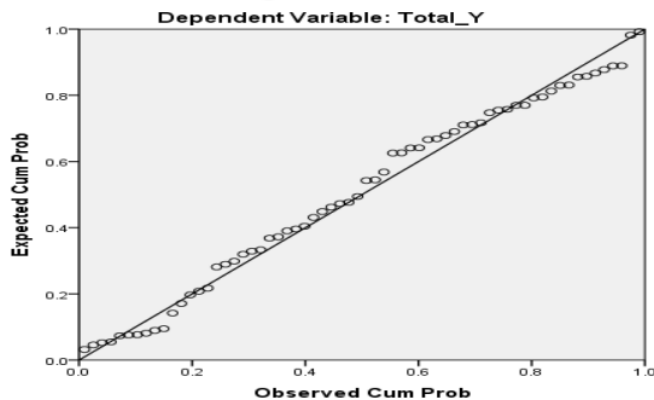
Gambar 1. Hasil Uji Normalitas – Normal Probability Plot Normal P-P Plot of Regression Standardized Residual
