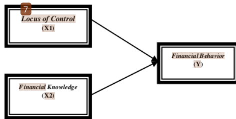
Fig.3.1: Research Model
