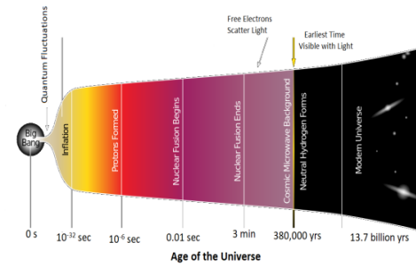
Figure 1: Age of the Universe Table 3: Summary of Cosmic Evolution
