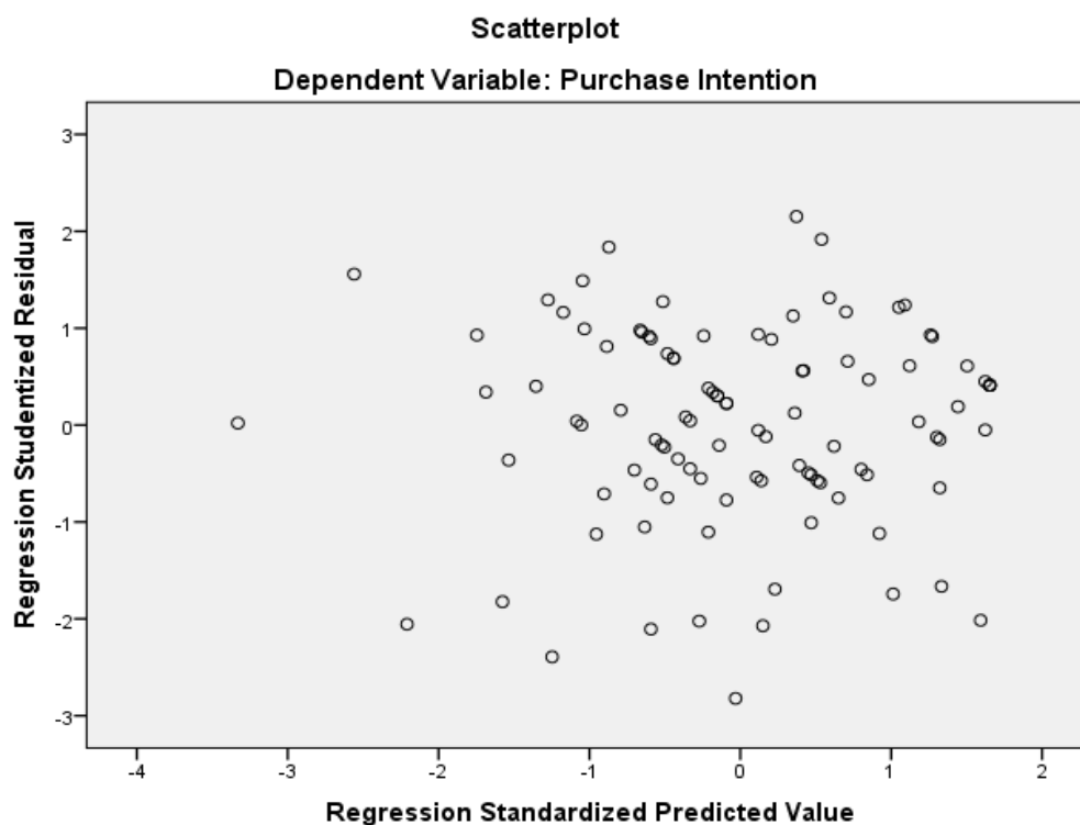
Gambar 4.1 Hasil Uji Scatterplot
