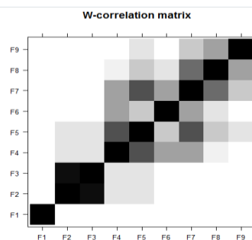
Gambar 4.3 Plot W-correlation
