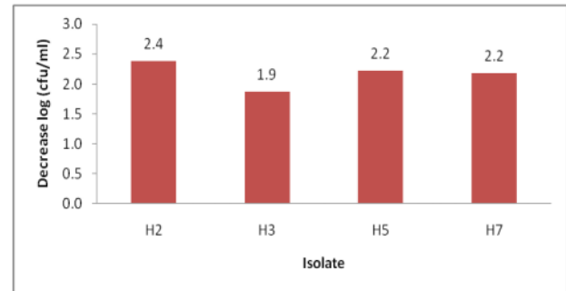
Figure 2. Resistance of bile salts to LAB isolates
