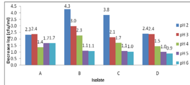
Figure 1. Resistance of isolate to various pH conditions
