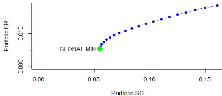
Gambar 4.1 Plot Global Minimum Portofolio
