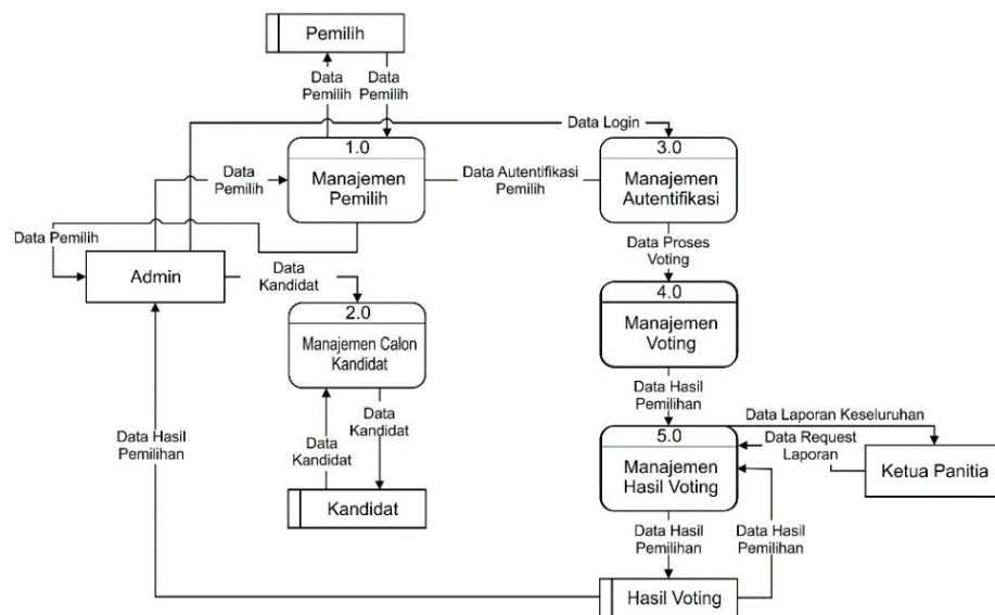
Gambar IV.5 DFD Level 1
