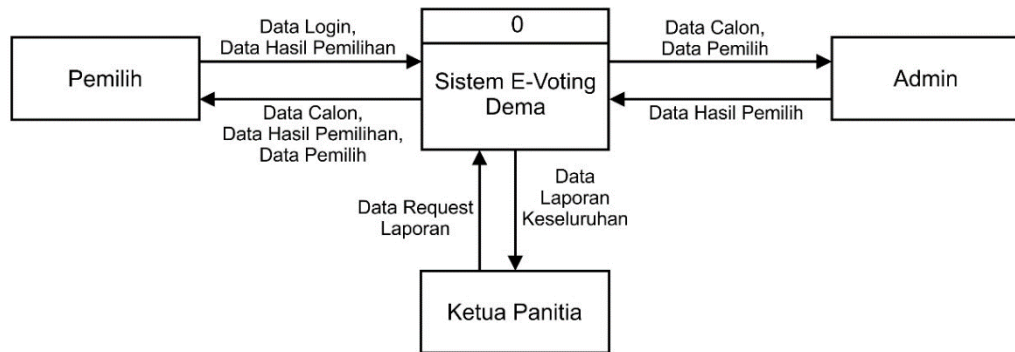
Gambar IV.4 Context Diagram
