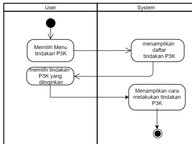
Gambar IV.6. Activity Diagram Tindakan P3K.
