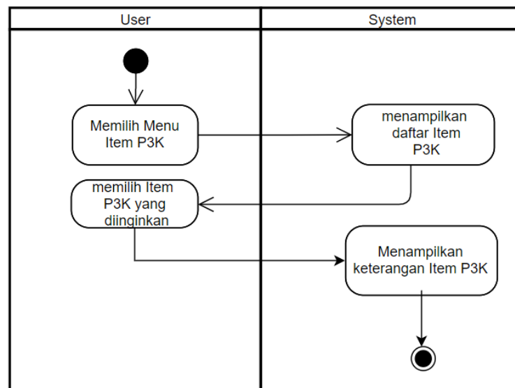
Gambar IV.8. Activity Diagram Item P3K.
