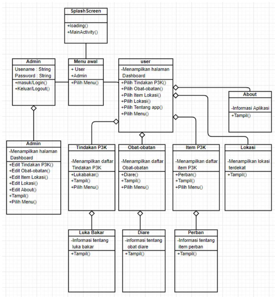
Gambar IV.18. Class Diagram
