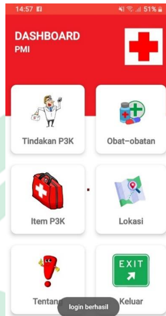
Gambar V.3. Antarmuka Dashboard.
