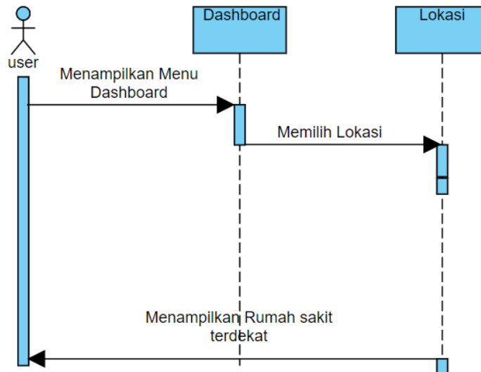
Gambar IV.15. Sequence Diagram Menu Lokasi
