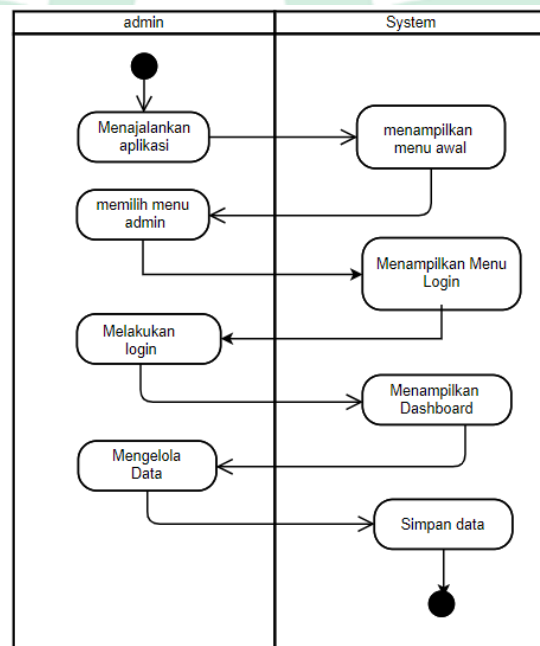
Gambar IV.5. Activity Diagram Admin
