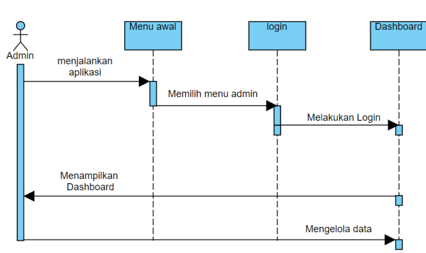
Gambar IV.17. Sequence Diagram Menu Admin
