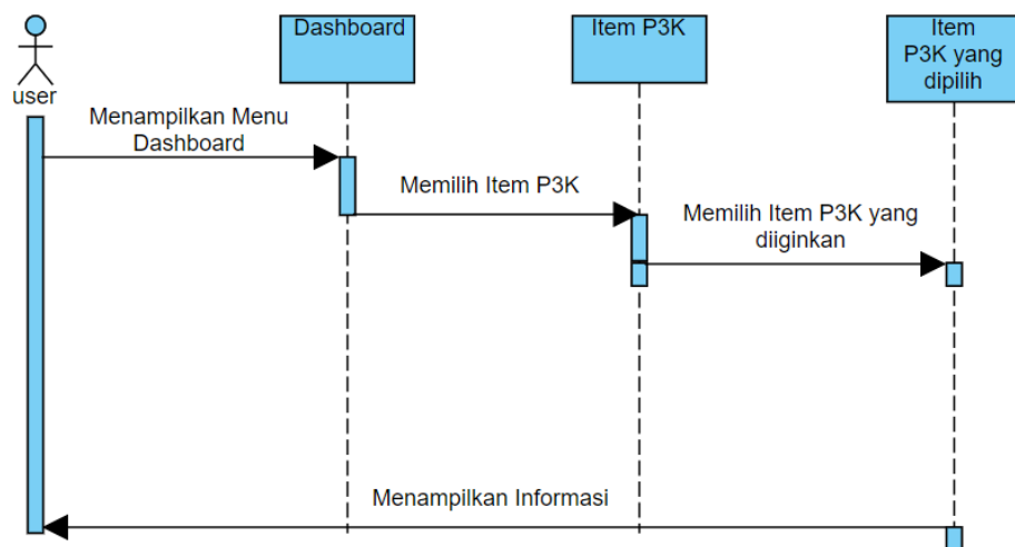
Gambar IV.14. Sequence Diagram Menu Item P3K
