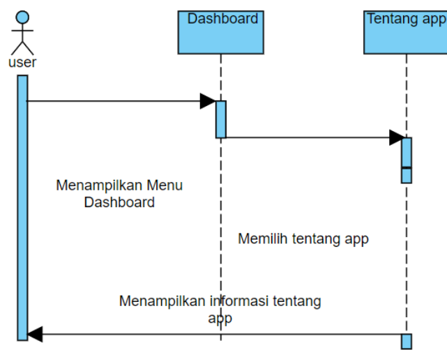
Gambar IV.16. Sequence Diagram Menu Tentang App
