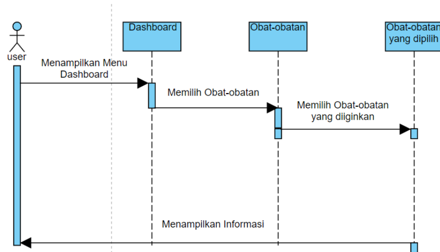
Gambar IV.13. Sequence Diagram Menu Obat-obatan
