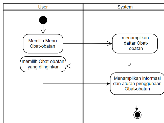
Gambar IV.7. Activity Diagram Obat-obatan
