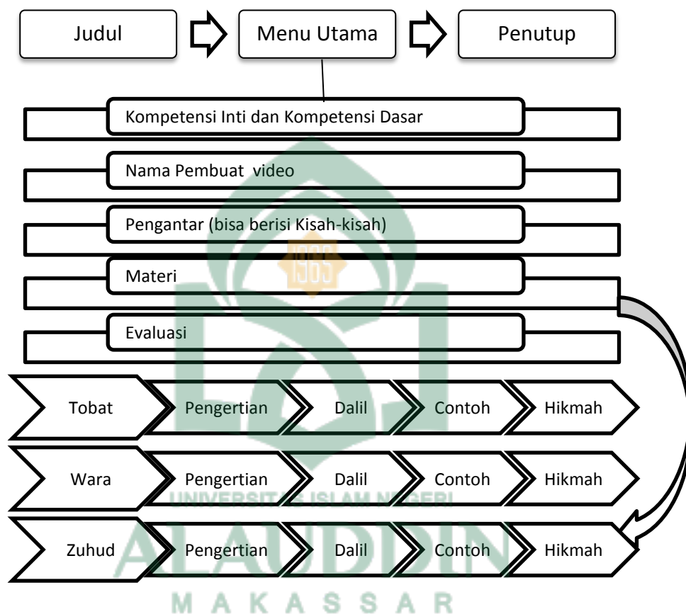
Gambar 2.11: Flowchart
