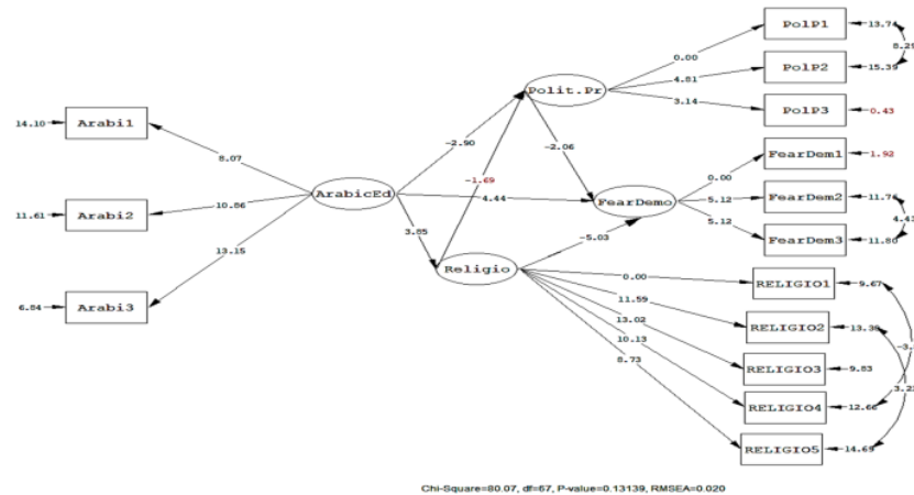
Figure 2. The t -value of the model (Source: Lisrel output).
