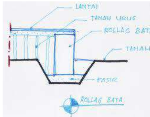
Gambar III.7 Pondasi Rollag Bata Sumber : www.mediaproyek.com , diakses september 2019
