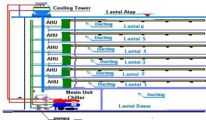
Gambar III.2 Sistem penghawaan AC central Sumber : http://www.electronicglobal.com , diakses september 2019
