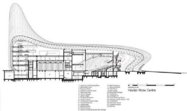
Gambar II.4 Detail Fungsi Heydar Aliyev Center
