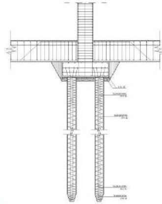
Gambar III.12 Pondasi tiang pancang
