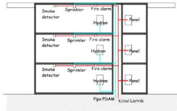
Gambar III.5 Sistem APAR Sumber : Hasil Analisis, 2019
