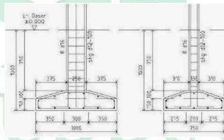
Gambar III.8 Pondasi poer Sumber : https://www.dataarsitek.com , diakses september 2019
