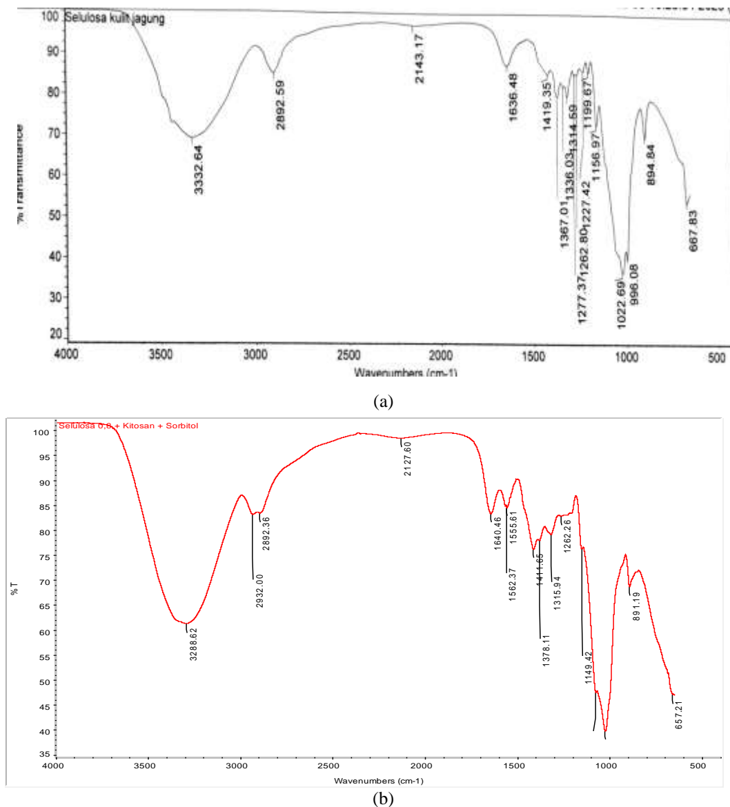
Gambar 4.6 (a) spektrum FTIR selulosa kulit jagung, (b) spektrum FTIR selulosa kulit jagung + kitosan + sorbitol
