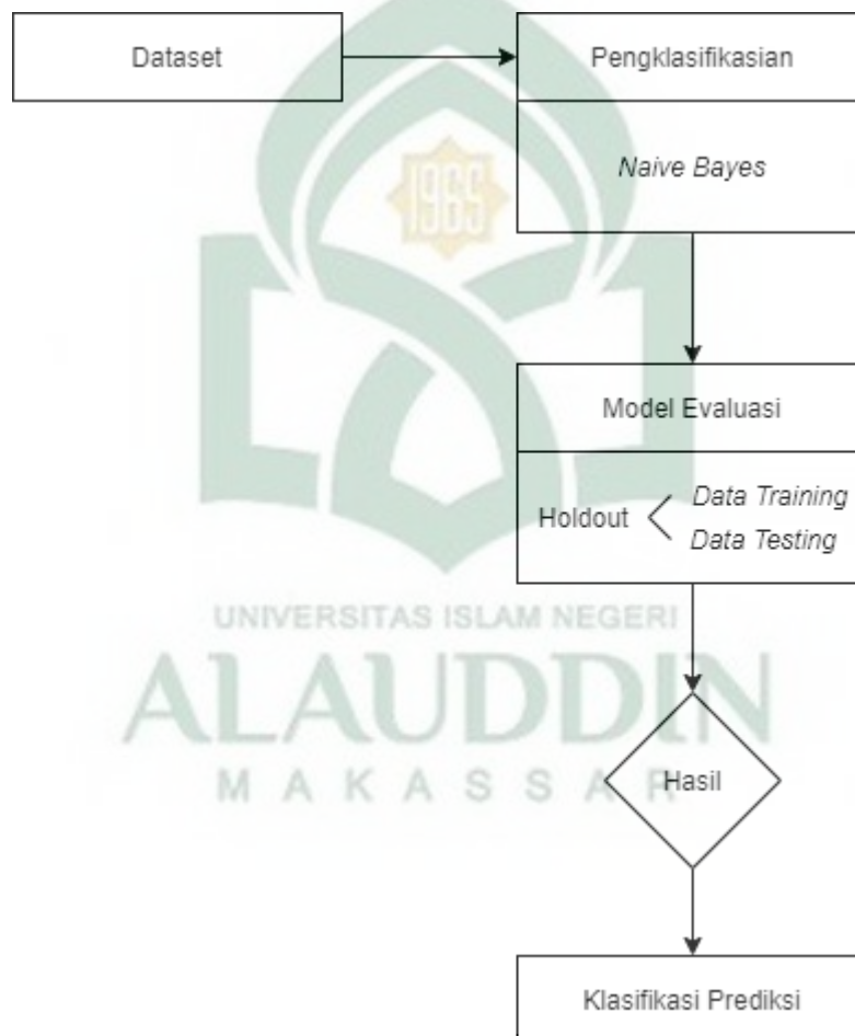
Gambar II. 1 Tahap Proses Algoritma Naive Bayes (Ting dkk, 2012: 39)
