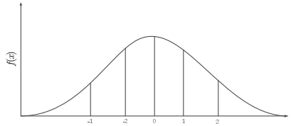
Gambar 1. Kurva Distribusi Normal Baku
