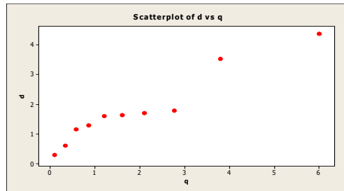
Gambar 5. Scatte plot data d v.s q
