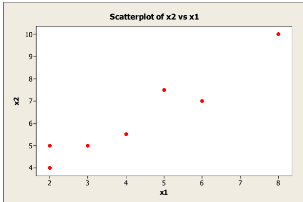
Gambar 1. Scatter plot variable x_1 dan x_2
