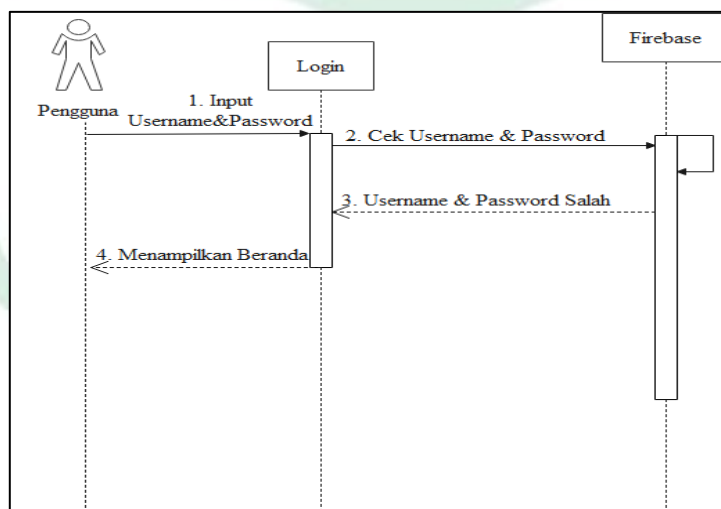
Gambar IV. 8. Sequence Diagram Login
