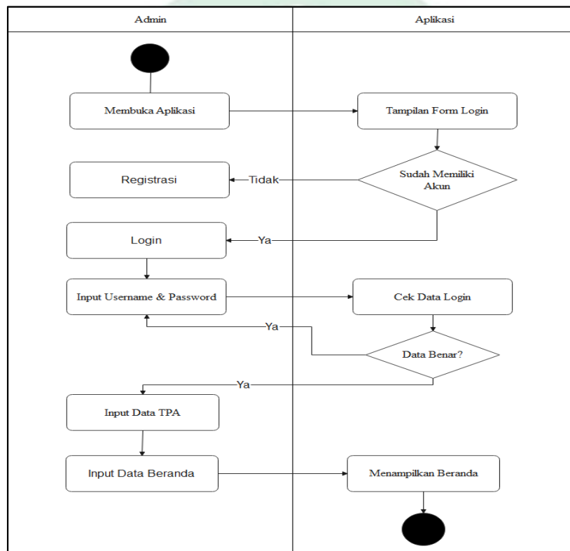
Gambar IV. 5. Activity Diagram Admin
