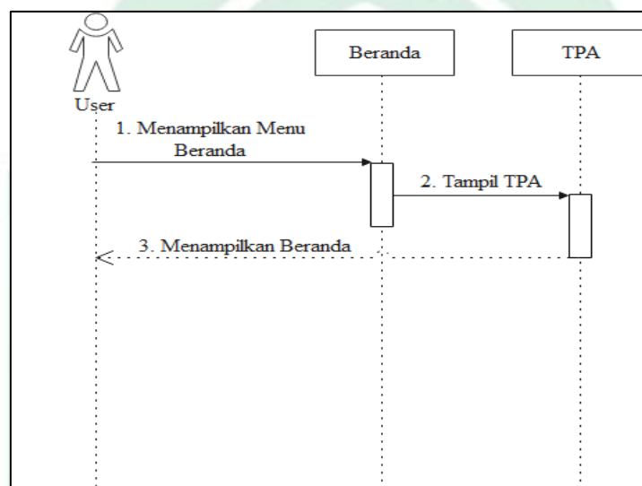
Gambar IV. 9. Sequence Diagram Beranda
