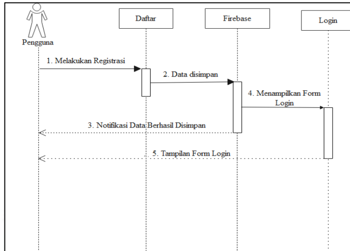
Gambar IV. 7. Sequence Diagram Registrasi
