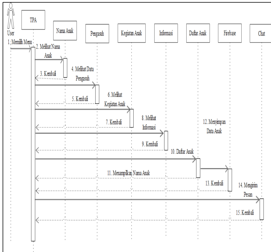
Gambar IV. 10. Sequence Diagram TPA
