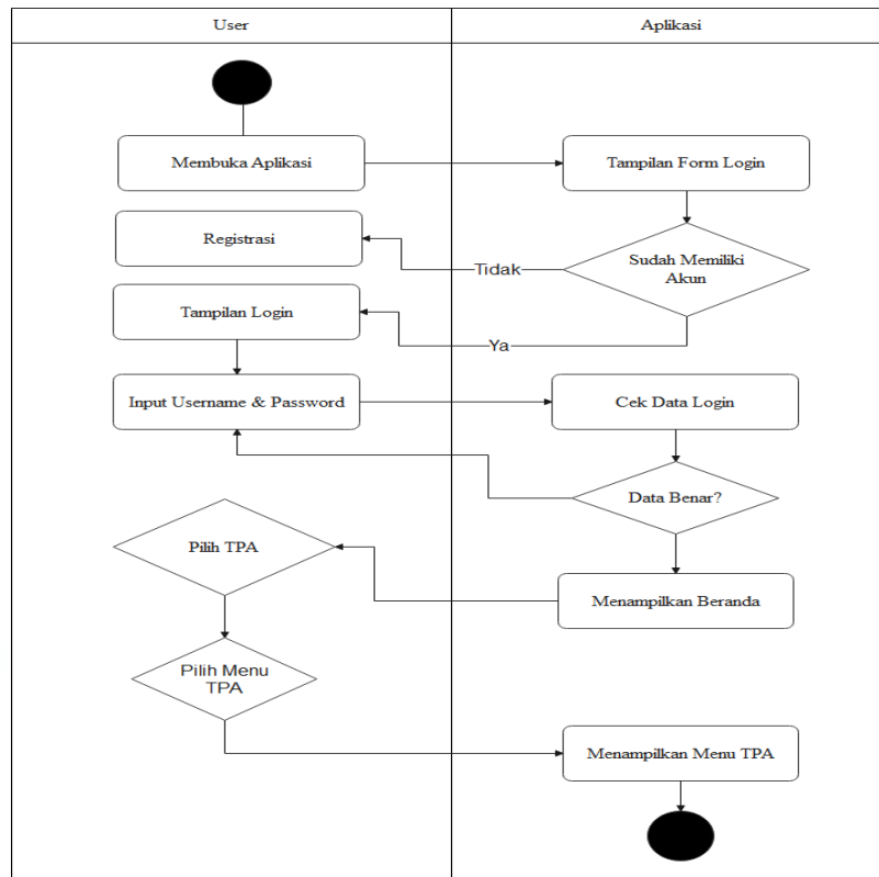
Gambar IV. 6. Activity Diagram User
