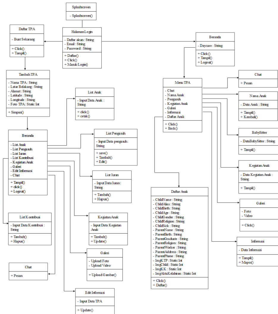
Gambar IV. 4. Class Diagram
