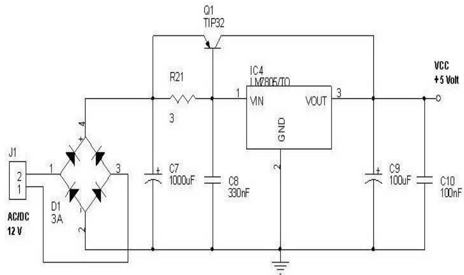
Gambar IV.5. Rangkaian Power Supply (Moch. Adib Musyafa, 2015).
