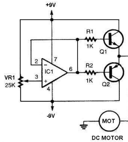
Gambar IV.6. Gambar Rangkaian Motor Servo (Yudi, 2015 )
