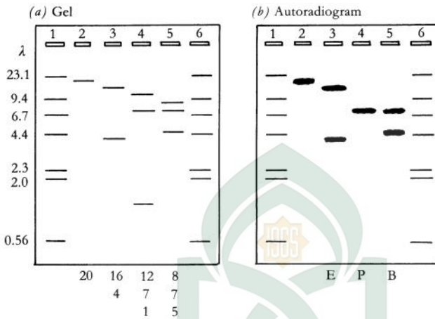
Gambar 6.2 Analisis Southern blotting
