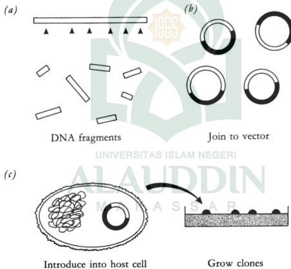
Gambar 1.3 Kloning Fragmen DNA (Desmond)
