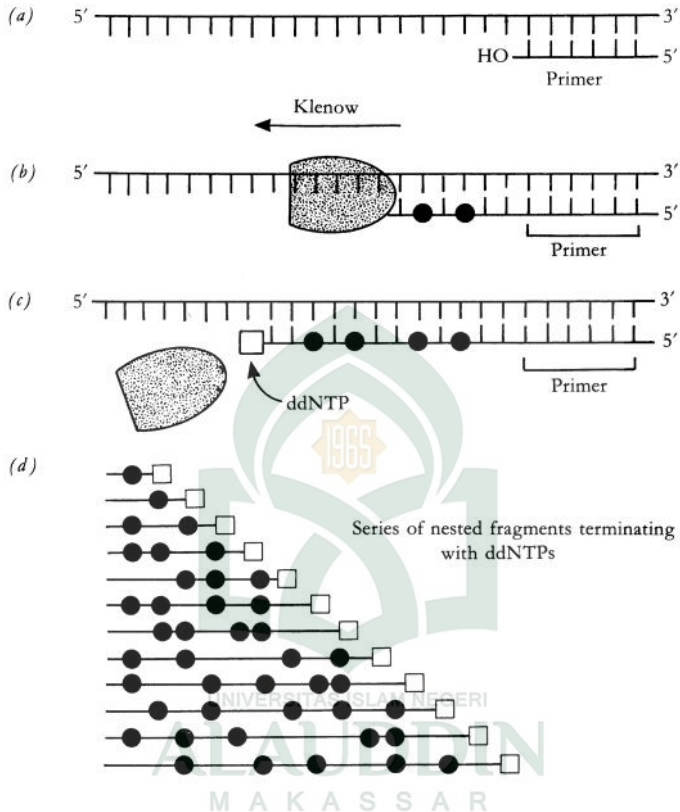
Gambar. 4.7 DNA sequencing using the dideoxy chain termination (Sanger–Coulson) method. (a) A primer is annealed to a single-stranded template and (b) the Klenow fragment of DNA polymerase I used to synthesise a copy of the DNA. A radiolabelled dNTP (often [ ^{35}\text{S} ]dNTP, filled circles) is incorporated into the DNA. (c) Chain termination occurs when a dideoxy nucleoside triphosphate (ddNTP) is incorporated. (d) A series of four reactions, each containing one ddNTP in addition to the four dNTPs required for chain elongation, generates a set of radiolabelled nested fragments.
