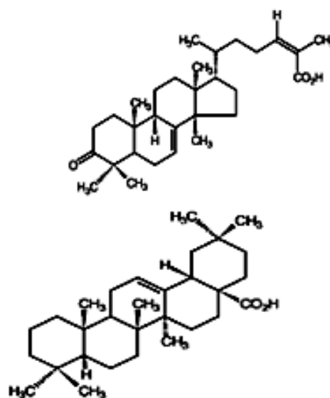
Fig. 1. Molecular structure of Triterpenoid Carbocsilat acid
