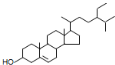
Fig. 2. The molecular structure of steroid compounds (-sitosterol)
