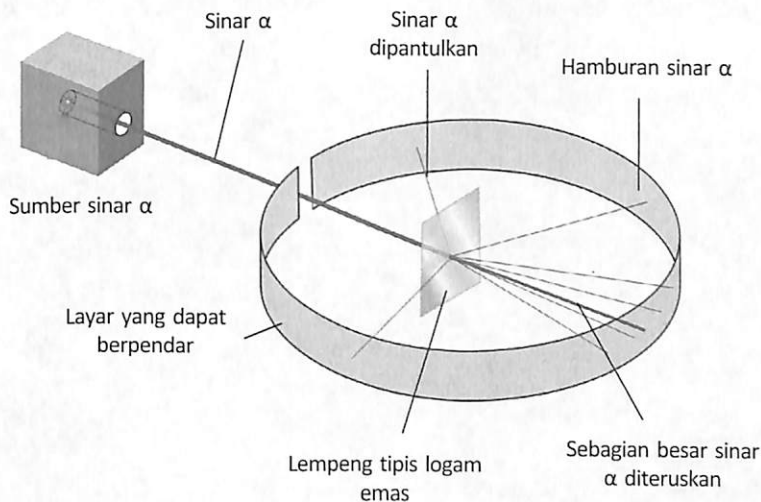
Gambar 3.3 Percobaan Rutherford
