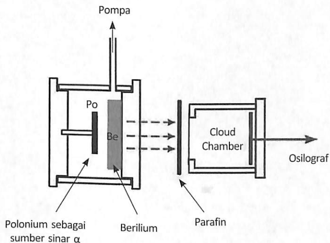
Gambar 3.4 Percobaan Chadwick
