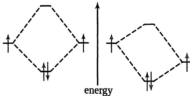
Gambar 8.1 Diagram MO
