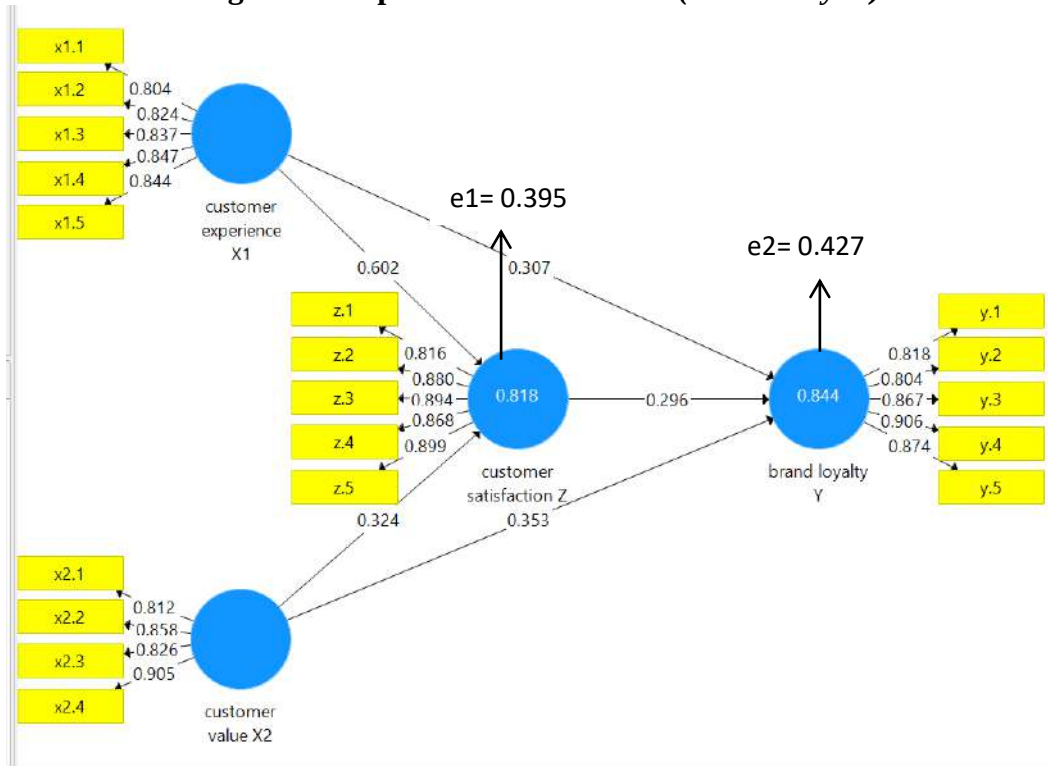
Gambar 4.2 Diagram Interpretasi Analisis Jalur ( Path Analysis )
