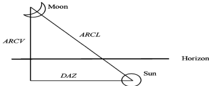
Figure 2. Fundamental geometry variable to predict hilal visibility
