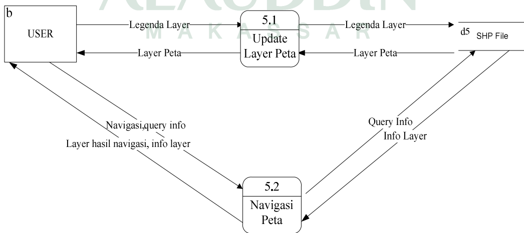
Gambar 4.9 DFD level 1 Proses Peta
