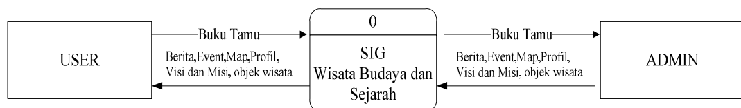
Gambar 4.4 Diagram Konteks
