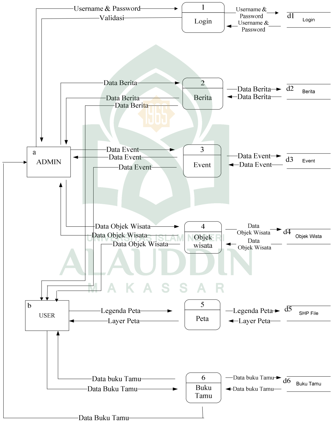
Gambar 4.5 DFD level 0
