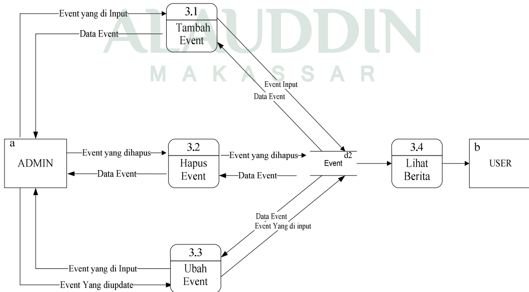
Gambar 4.7 DFD level 1 Proses Event
