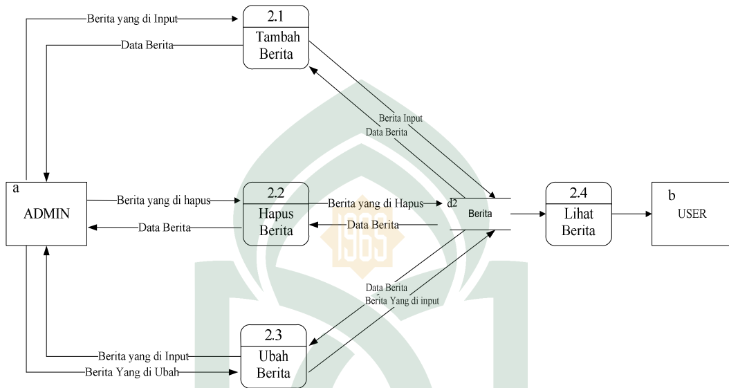
Gambar 4.6 DFD level 1 Proses Berita
